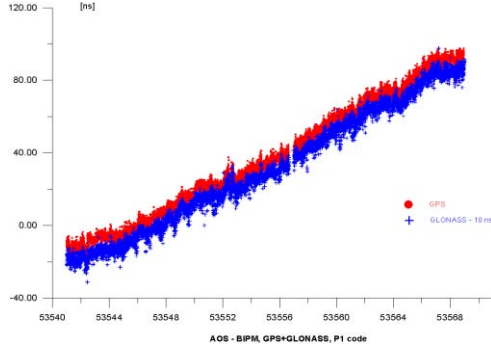
Figure 4. Comparison of clocks between AOS and BIPM, distant by 1200 km, using GPS and GLONASS time transfer.
