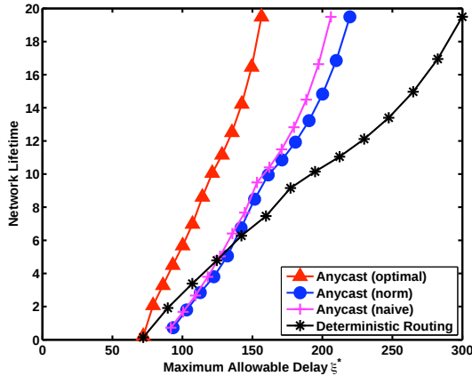
Fig. 4. The network lifetime according to different allowable delay \xi^* when nodes are not uniformly distributed.
