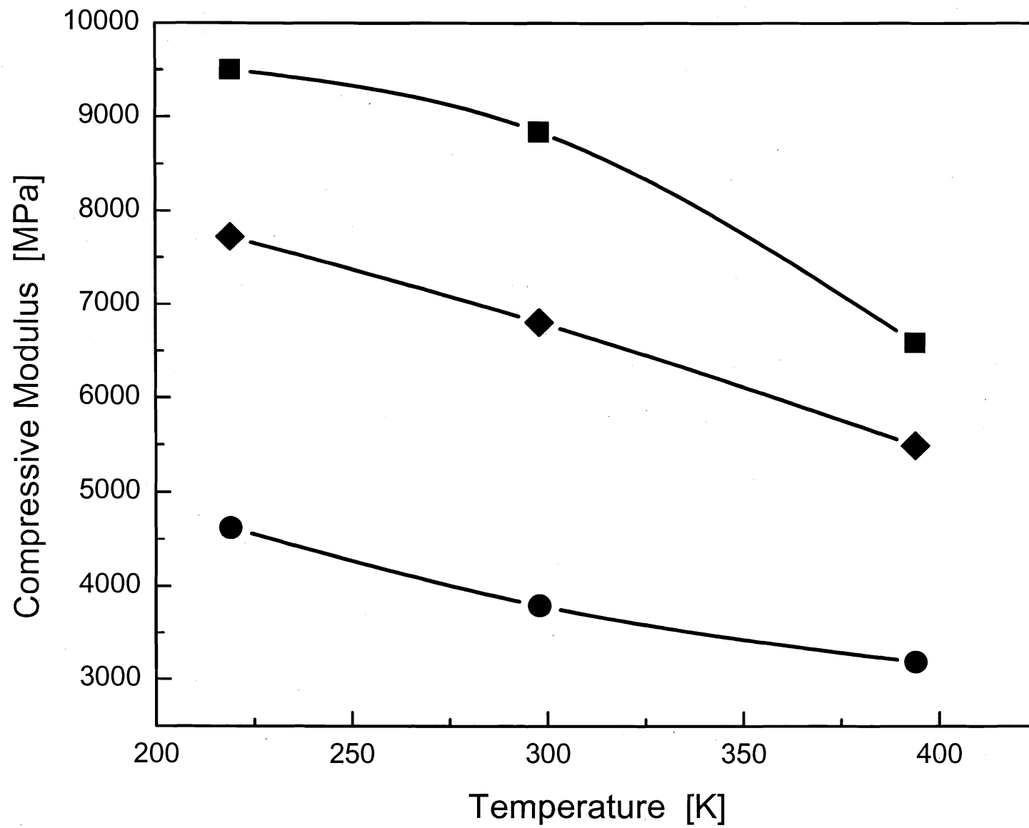
Fig. 7A: Exptl. Compressive Modulus of Parmax SRPs
