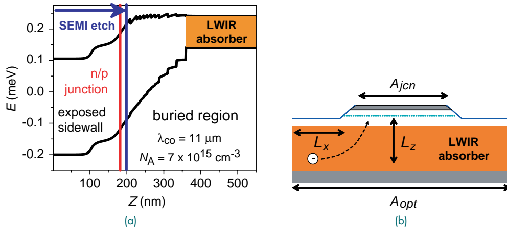
FIGURE 5 SEMI process for graded bandgap T2SL photodiodes: (a) bandstructure; (b) schematic of photodiode cross-section. A_{jcn} = junction area; A_{opt} = optical area; L_x = lateral diffusion length; L_z = vertical diffusion length.
