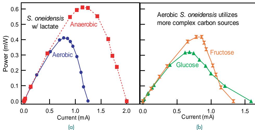
FIGURE 3 (a) Power versus current plot demonstrating for the first time that MFCs can generate power in completely aerobic environments. Power output dropped by roughly 30% due to oxygen scavenging of electrons in the anode chamber. (b) Power versus current plot demonstrating how S. oneidensis utilizes sugars to generate electricity under aerobic conditions.
