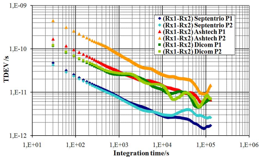
Figure 6. Time deviation of the P-code difference.
