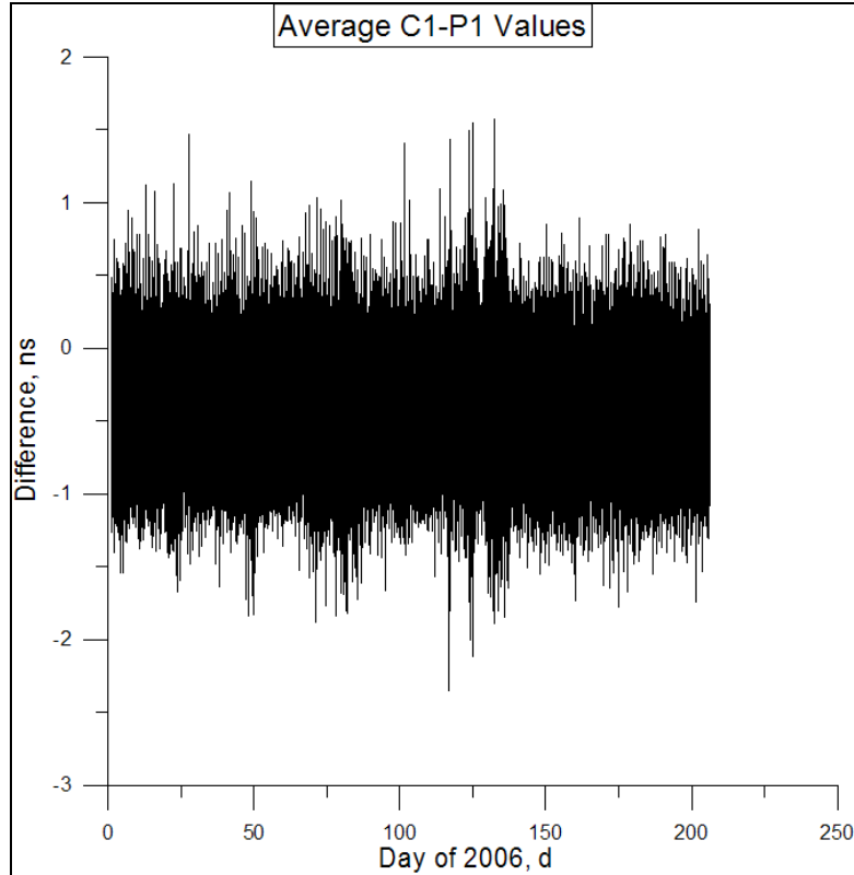
Figure 1. C1-P1 values averaged over typically nine satellites. The mean was -0.414 ns.
