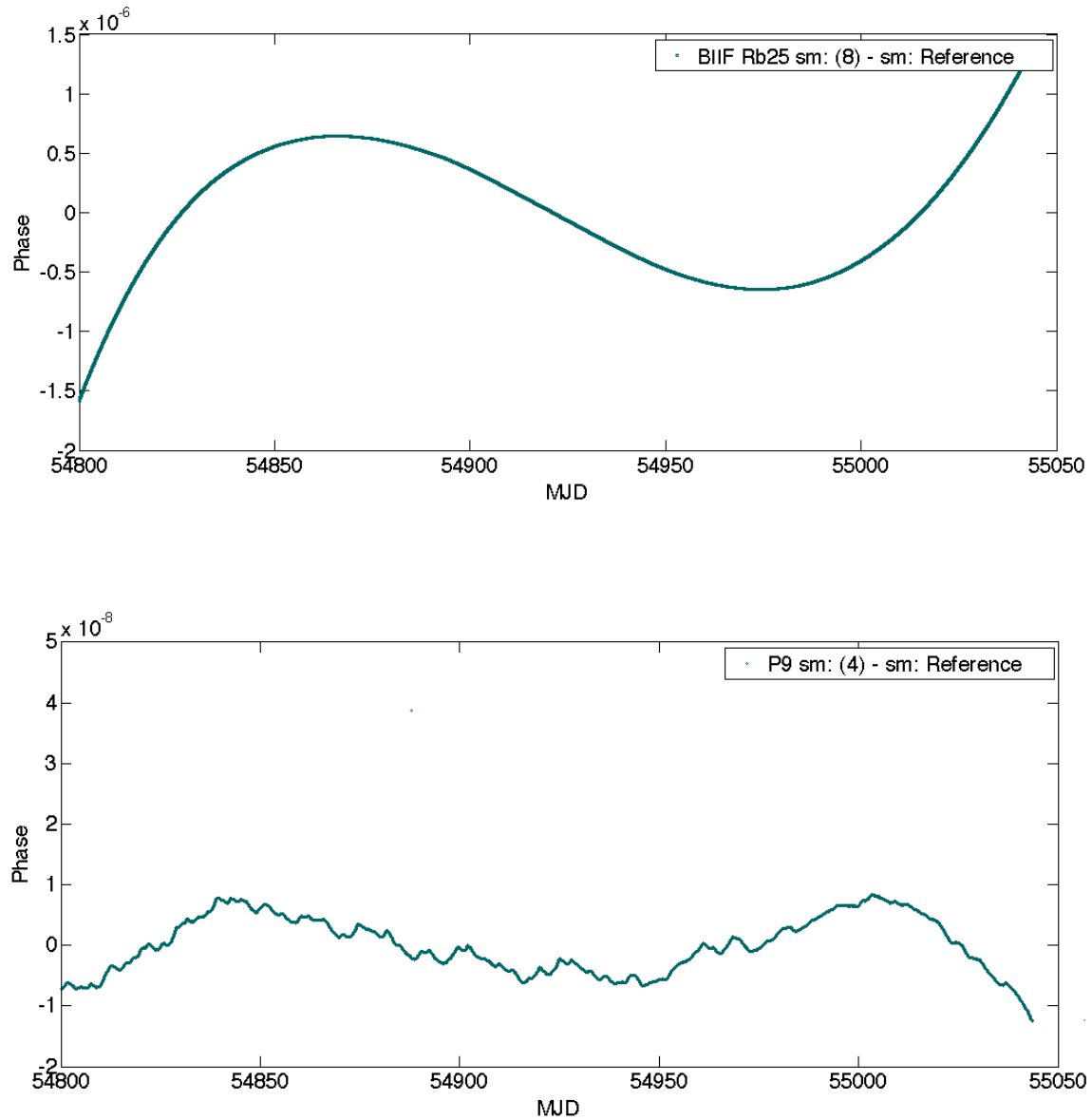
Figure 4. Remove Trend Line. The phase data trend line for both plots is removed. This allows the data to be more closely inspected to determine if the phase breaks have been removed.
