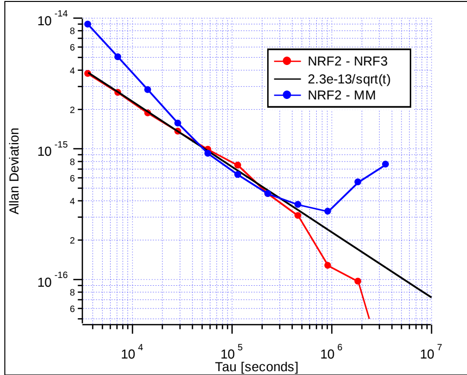
Figure 4. Performance of rubidium fountains NRF2 and NRF3 against each other, and against a USNO maser mean. The straight line segment is a fit to the inverse square-root curve expected for white frequency noise. The subdaily statistics are contaminated by switch measurement noise, while the large-tau statistics have a high uncertainty.
