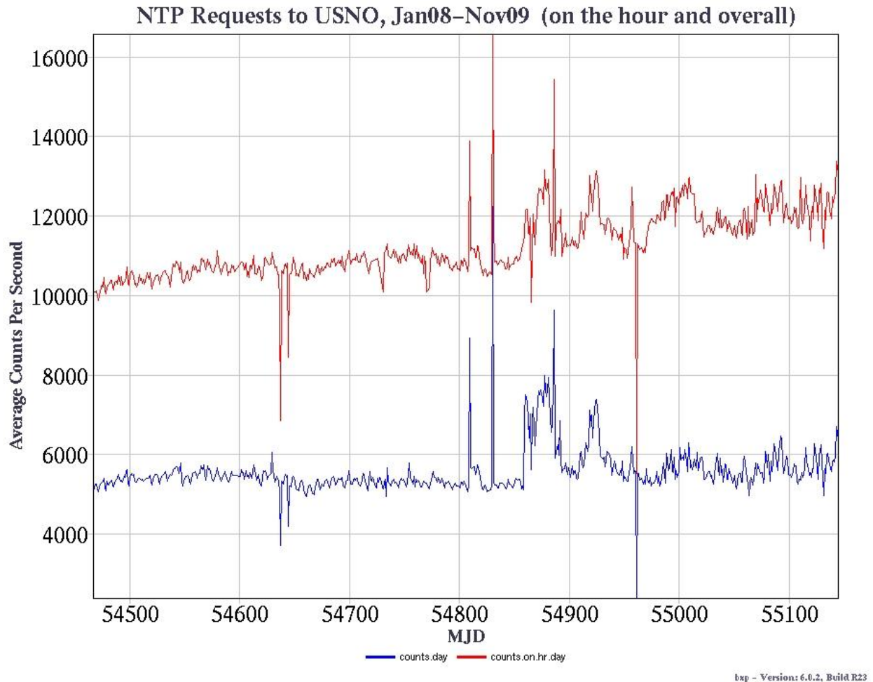
Figure 8. Measured NTP request rates to Washington DC servers since 2008. The upper plot is the request rate on the first second of every hour, which is the time when most clients are configured to query. The lower plot is the request rate averaged over the hour. The increase in February 2009 was due to a software modification.
