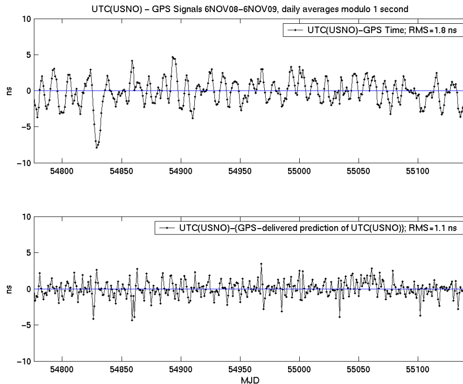
Figure 9. Recent daily averages of UTC (USNO) minus GPS Time and UTC minus GPS's delivered prediction of UTC (USNO).
