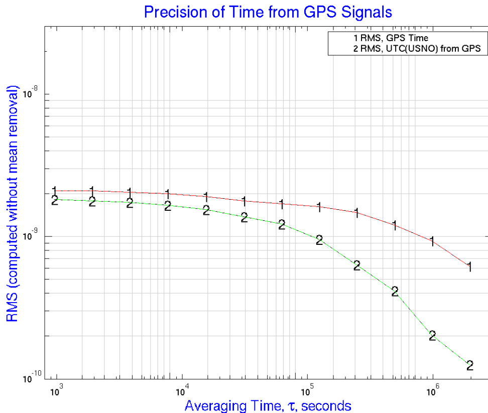
Figure 10. The precision of GPS Time and of GPS's delivered prediction of UTC (USNO), using TTR-12 data since 12 July 2002, measured by the attainable external precision (rms, mean not removed) as a function of averaging time, and referenced to UTC (USNO). Improved performance in accessing UTC (USNO) could be realized if only the most recently updated navigation messages are used. The accuracy attainable over a given averaging time also depends upon the calibration of the user's receivers.
