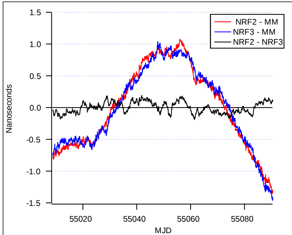
Figure 5. Slope-removed data which form the basis for the previous figure. The two rubidium fountains (NRF2 and NRF3) stay with 200 ps of each other while the USNO Maser Mean deviates by 1.5 ns from both.
