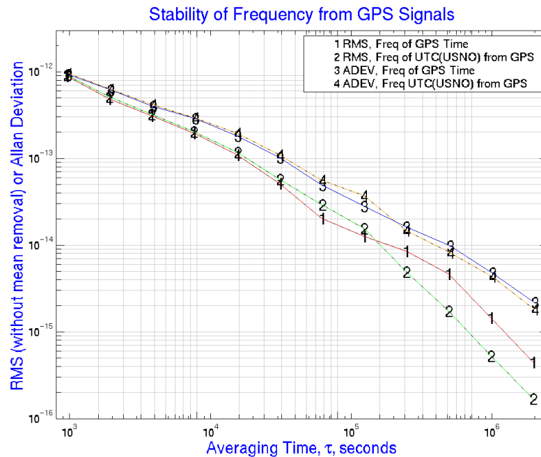
Figure 11. RMS fractional frequency external precision and the fractional frequency stability, as measured by the Allan deviation, of GPS Time and for GPS's delivered prediction of UTC (USNO), using TTR-12 data since 7 February 2005. The reference frequency is that of UTC (USNO).
