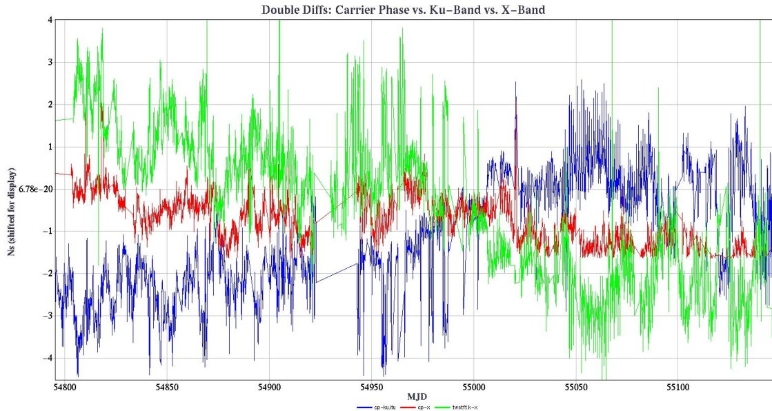
Figure 13. Double-differences of three time transfer links between USNO and PTB over the past year. The blue link is carrier-phase GPS difference with Ku-band TWSTT, the red is carrier-phase GPS differenced with X-band TWSTT, and the green is the difference between X-band and Ku-band TWSTT. The data gap is due to the GPS receiver's being moved to a more temperature-stable room. Curves were shifted for display.
