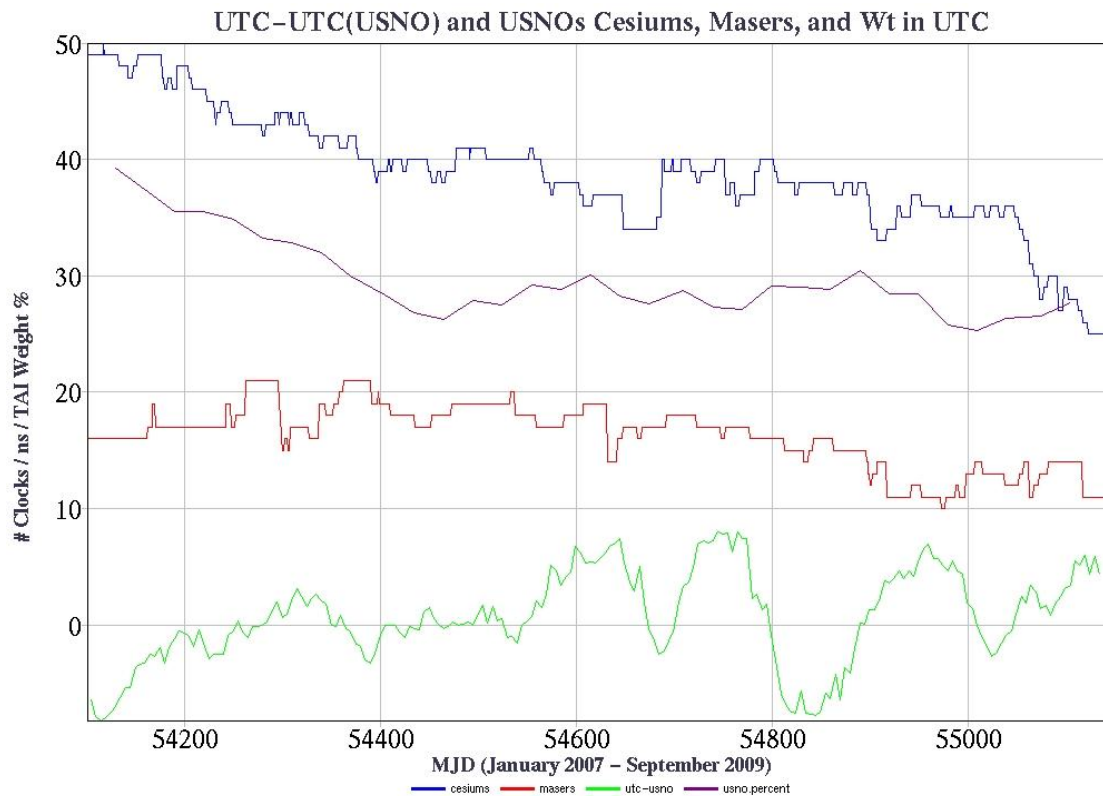
Figure 2. Recent trends, which may not be directly correlated. The highest plot is the number of USNO cesium 5071s used to compute the steering timescale. The next highest plot, solid line, is the total weight of USNO clocks in UTC generation (including AMC). The third plot is the number of cavity-tuned masers used in the USNO steering timescale, and the lowest plot is UTC – UTC (USNO).
