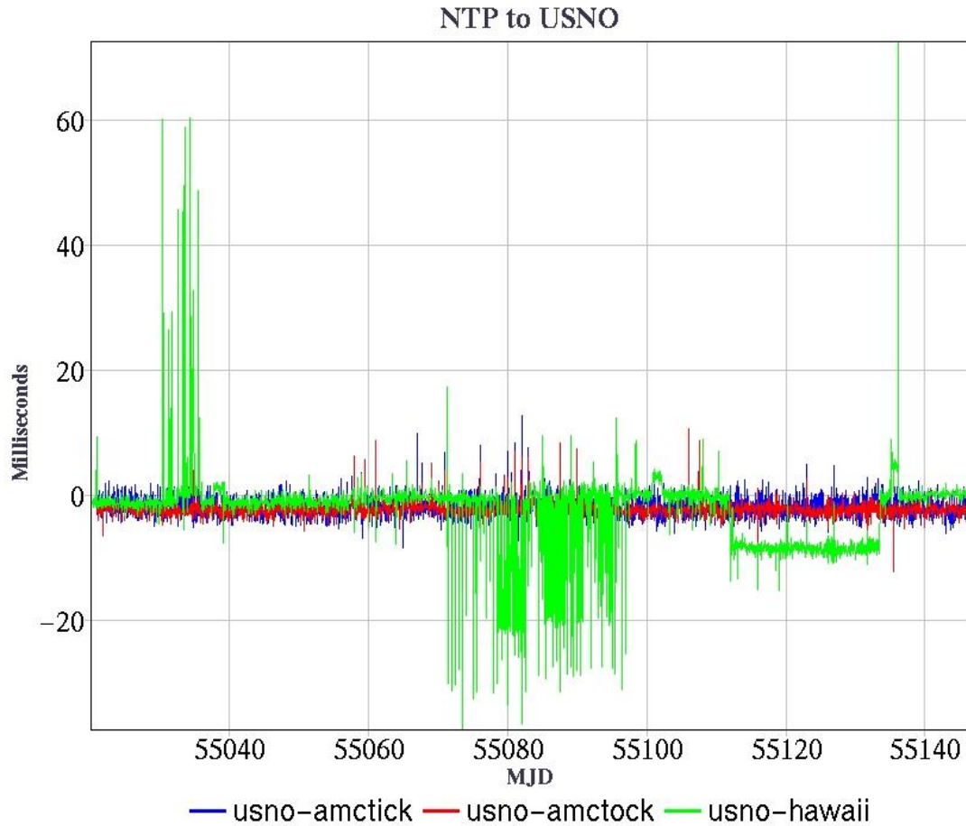
Figure 7. Time difference measured via NTP between USNO-DC and servers in Hawaii and AMC, which are 2500 miles apart. Plot is intentionally scaled so as to emphasize outliers associated with long-distance NTP. Clients on Hawaii would be expected to observe large outliers when accessing the Washington DC server, not their local one. Similarly, CONUS clients west of the Mississippi would attain greater precision by querying the AMC server instead of the Washington, DC one.
