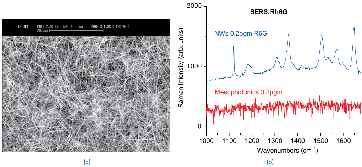
FIGURE 8 (a) Ga 2 O 3 core/Ag shell nanowire composite and (b) comparison of SERS signal for Mesophotonics “Klarite” commercial substrate and Ga 2 O 3 /Ag nanowires.
