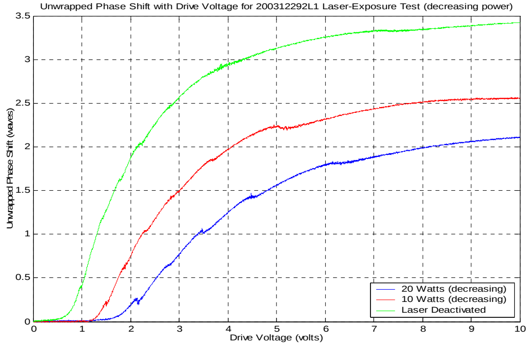
Figure 7: Unwrapped phase shift for laser-exposure test of phase shifter 200312292 (decreasing power).
