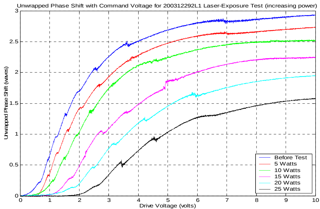
Figure 5: Unwrapped phase shift for laser-exposure test of phase shifter 200312292 (increasing power).
