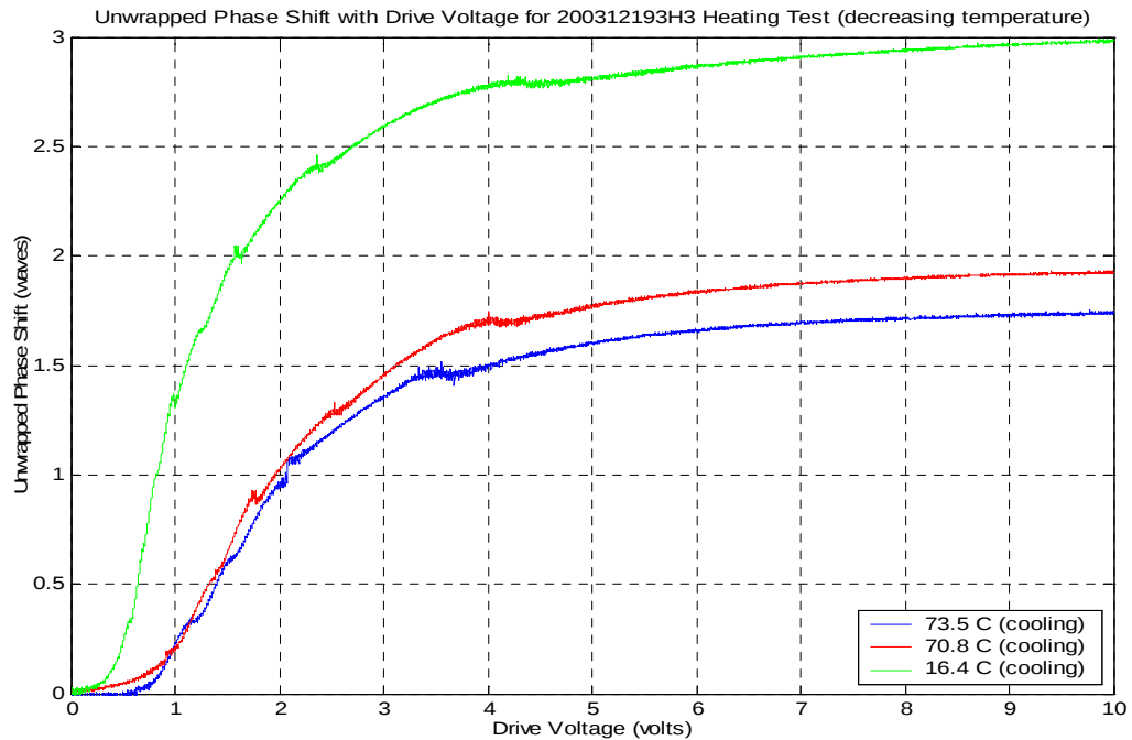
Figure 21: Unwrapped phase shift for H3 heating test of phase shifter 200312193 (decreasing temperature).
