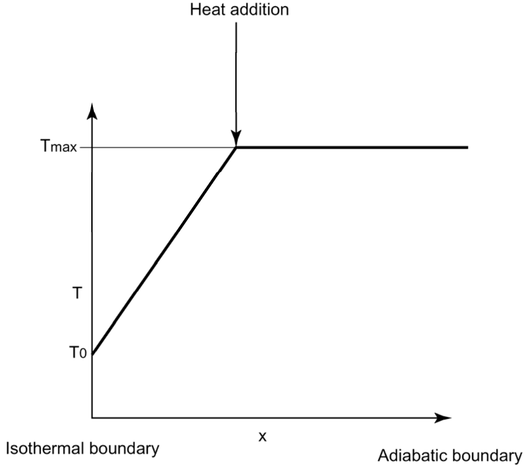
Figure 32: Simplified heat profile in an LCOPA device with one adiabatic boundary, one isothermal boundary, and heat addition taking place in a thin layer.
