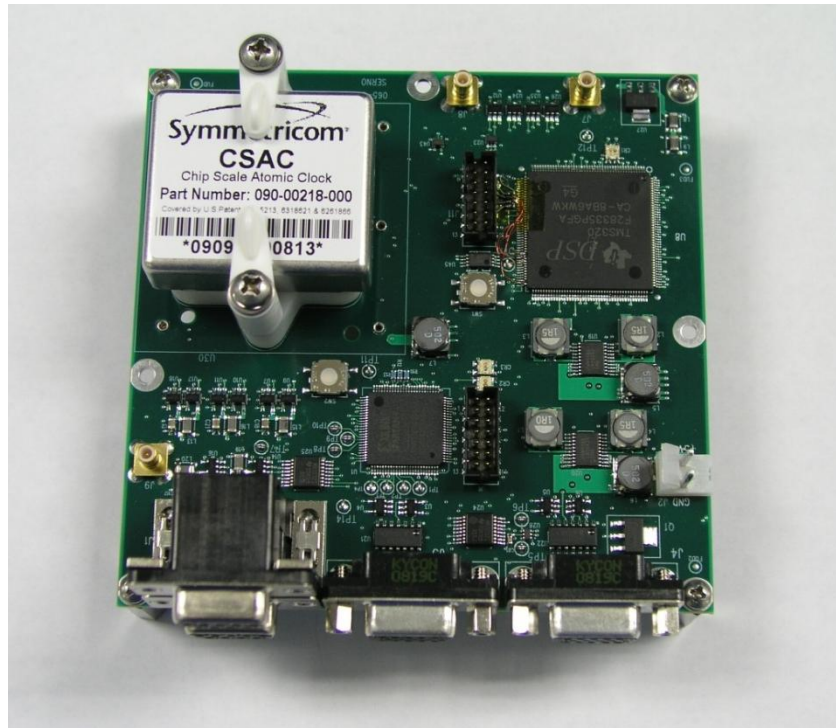
Figure 3. CTM Phase II Time Engine breadboard.
