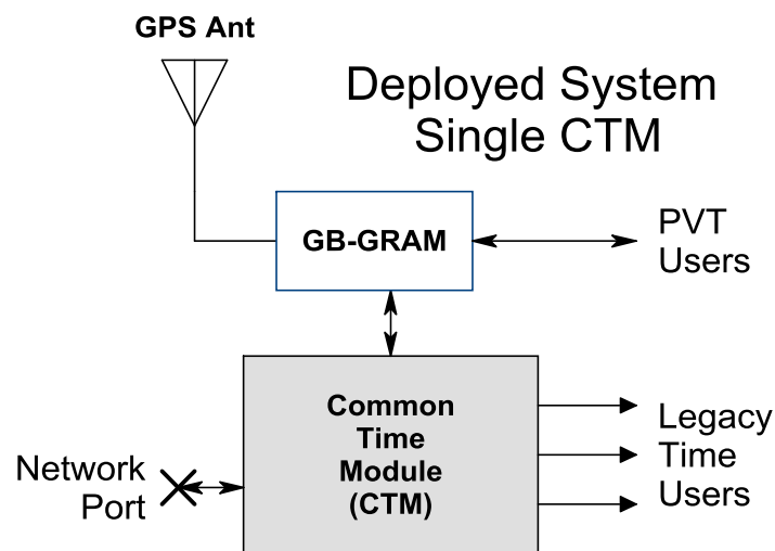
Figure 1. Simple CTM system deployment.
