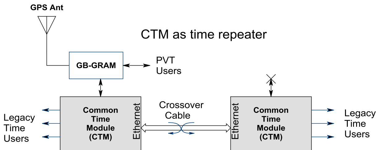
Figure 5. Remote CTM.
