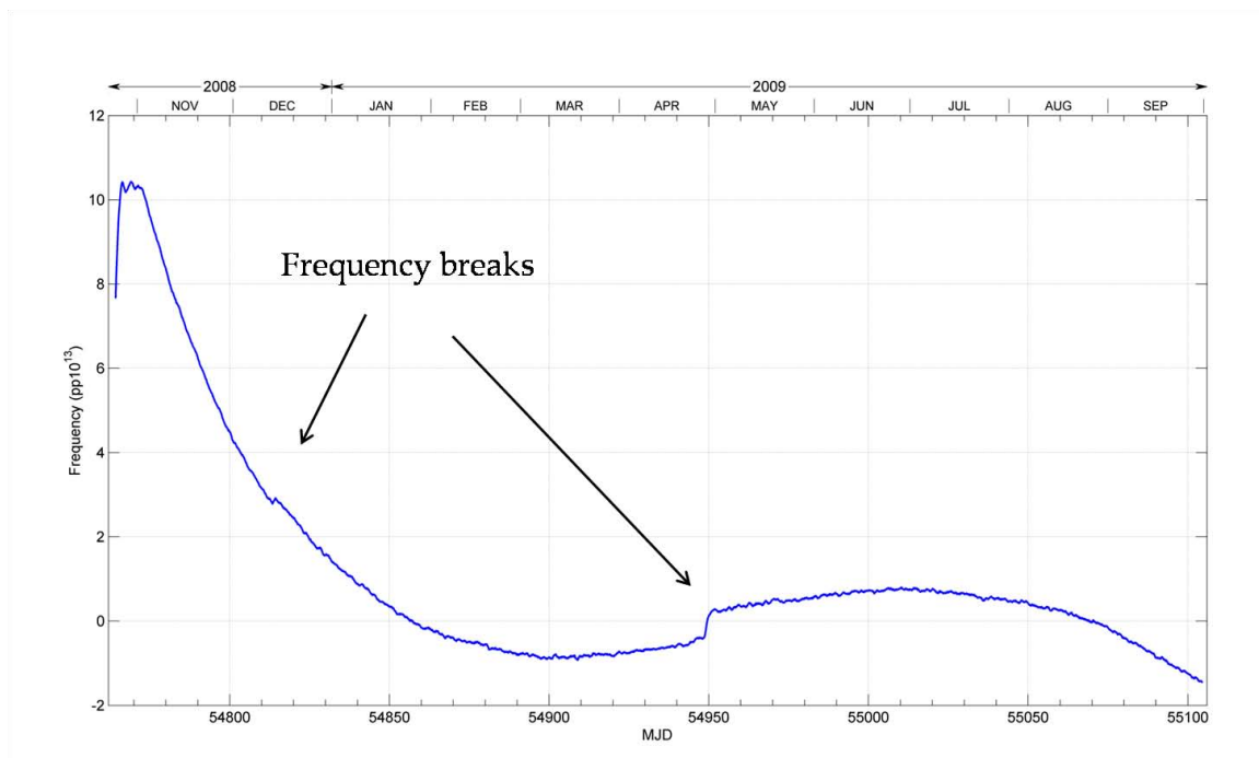
Figure 3. RFS SN05 average daily frequency offset residuals.
