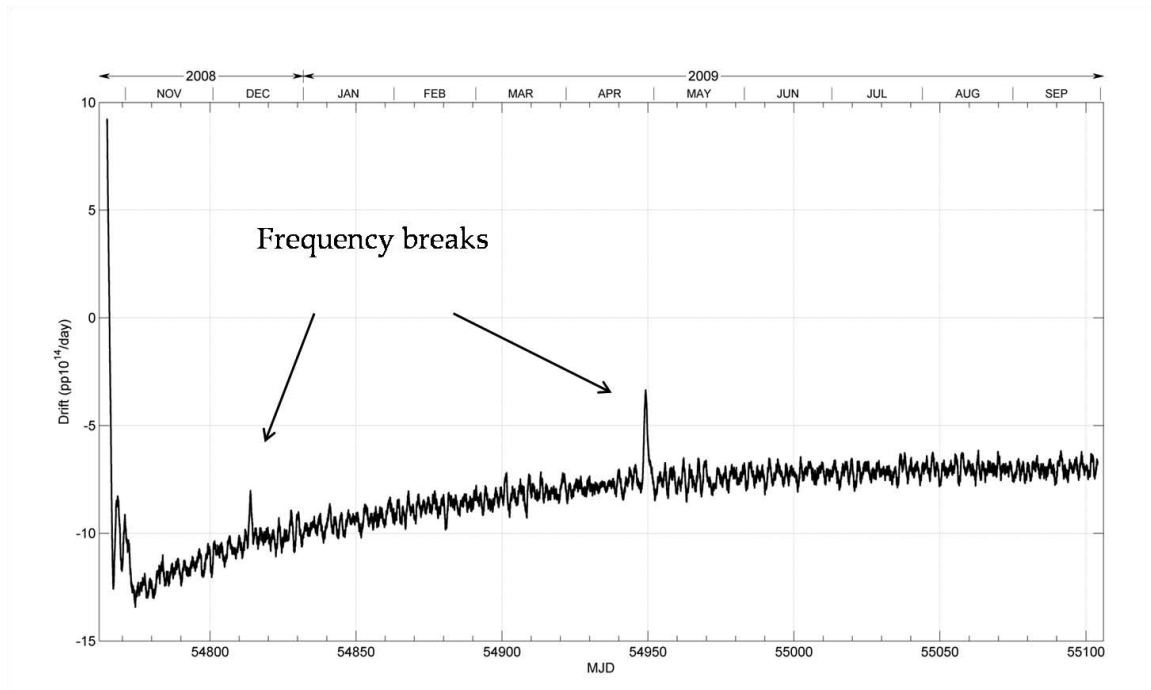
Figure 5. RFS SN05 daily drift offset.
