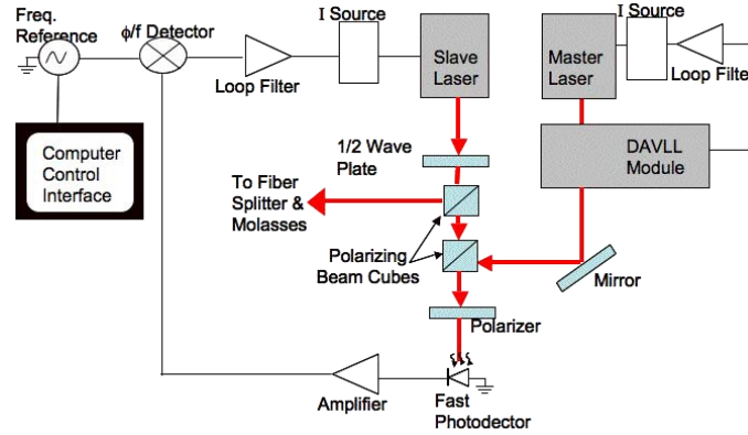
Figure 1. Diagram of offset-locking scheme.
