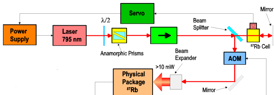
Figure 3. Optical Unit architecture.
