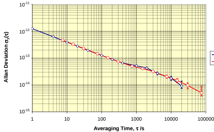
Figure 8. Frequency stability of the POP clock.
