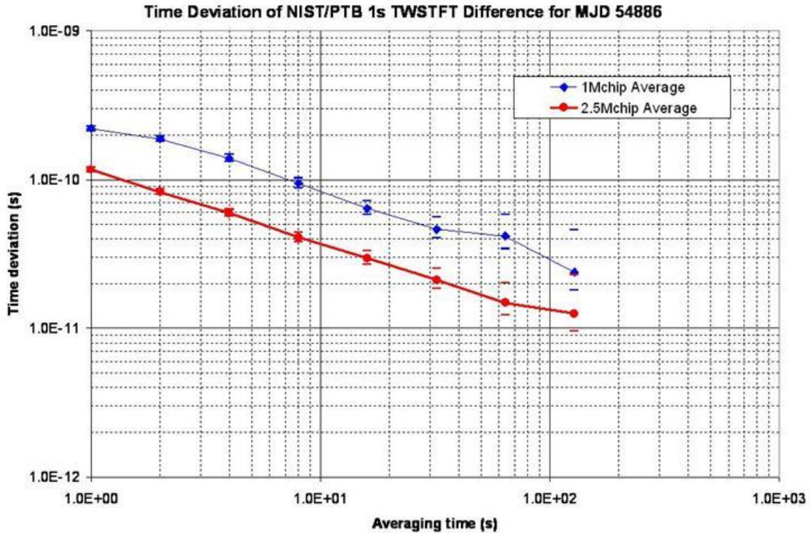
Figure 3. Short-term stability of the NIST/PTB TWSTFT.
