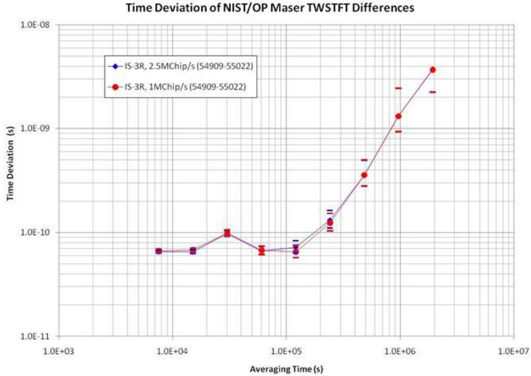
Figure 7. NIST/OP 1 MChip/s and 2.5 MChip/s long-term stability using the IS-3R satellite.
