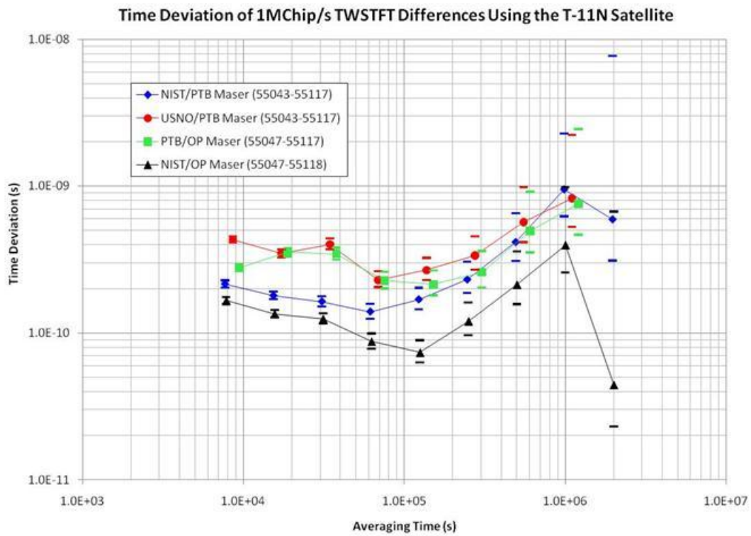
Figure 9. Long-term stability of the 1 MChip/s TWSTFT using the T-11N satellite.
