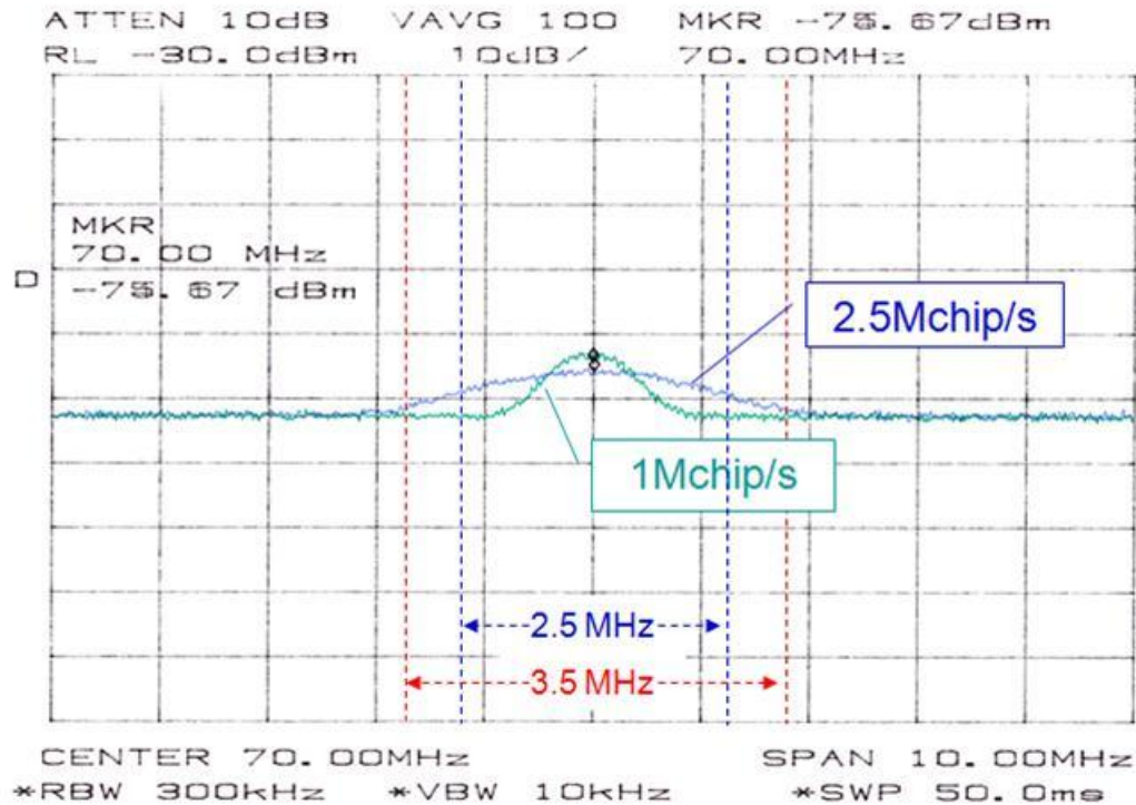
Figure 2. 1 MChip/s and 2.5 MChip/s RX IF spectrum signals.
