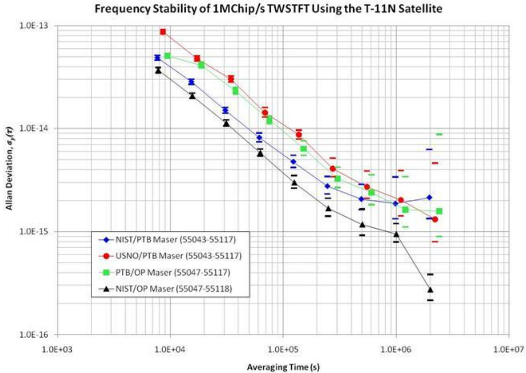
Figure 10. Frequency stability of the 1 MChip/s maser-to-maser TWSTFT using the T-11N Satellite.
