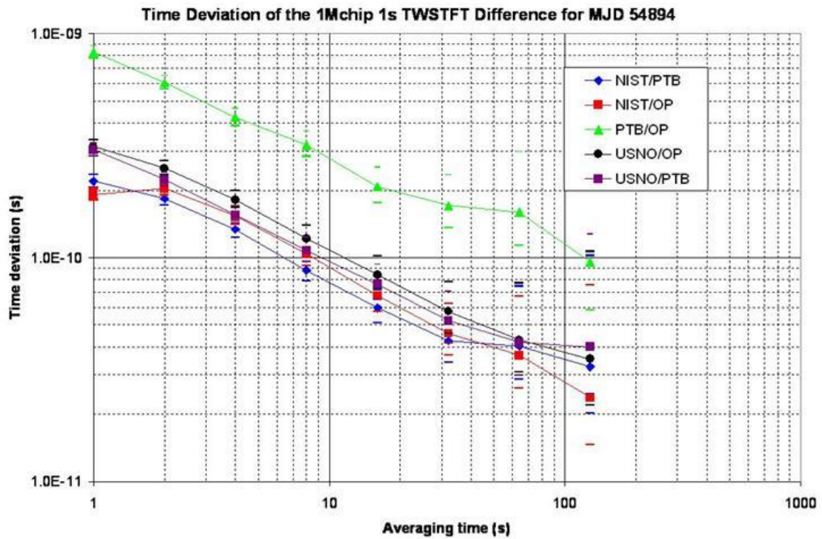
Figure 4. Short-term stability of the transatlantic and Europe-to-Europe 1 MChip/s TWSTFT
