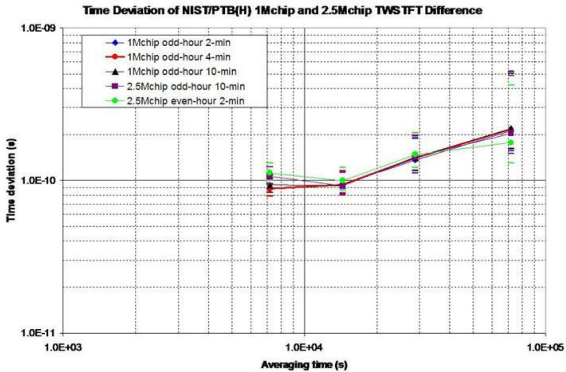
Figure 6. Time deviation of NIST/PTB TWSTFT with different measurement lengths.
