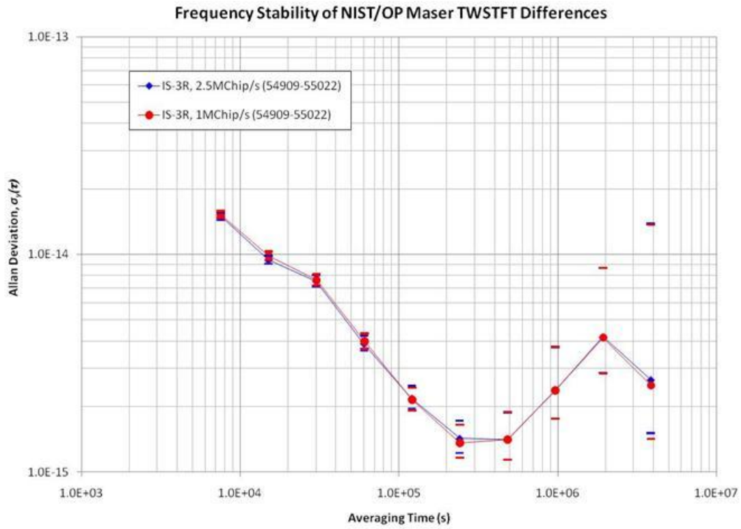
Figure 8. Frequency stability of the NIST/OP maser-to-maser 1 MChip/s and 2.5 MChip/s TWSTFT.
