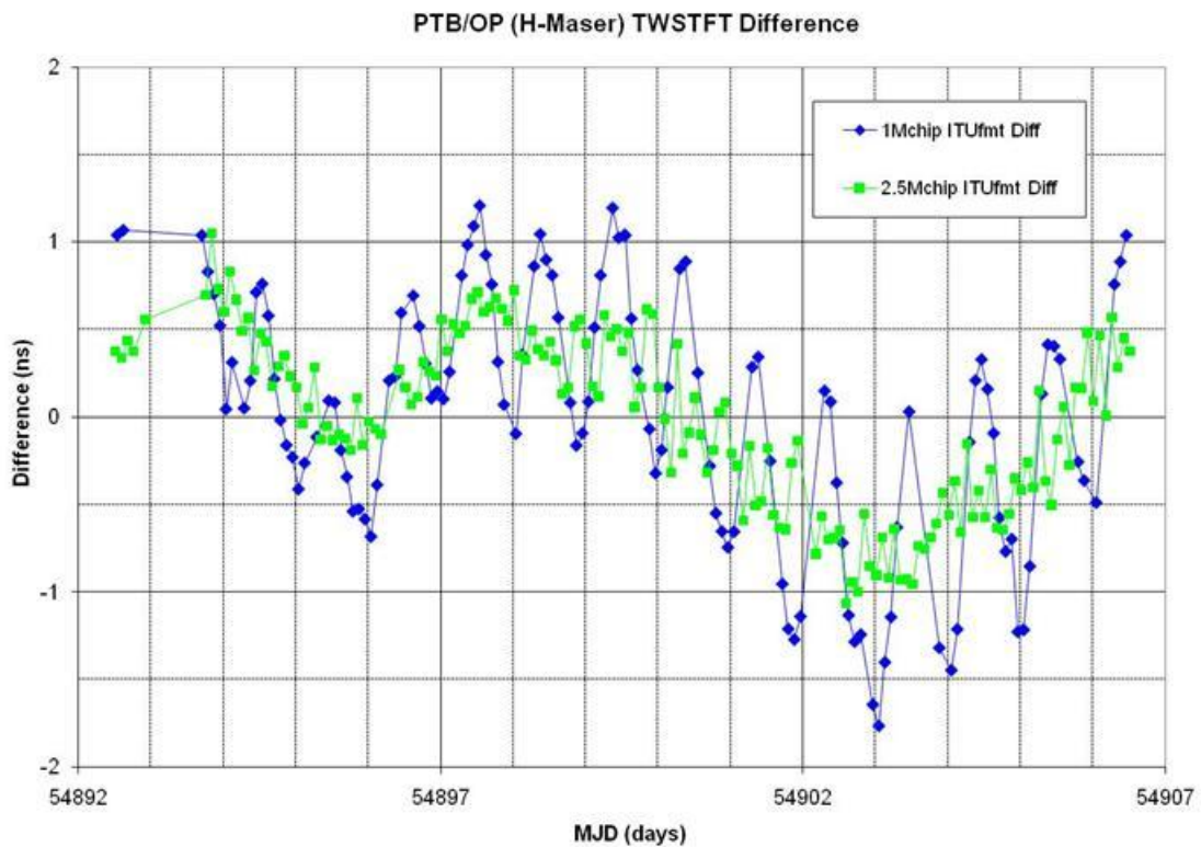
Figure 5. TWSTFT differences of the PTB/OP link.
