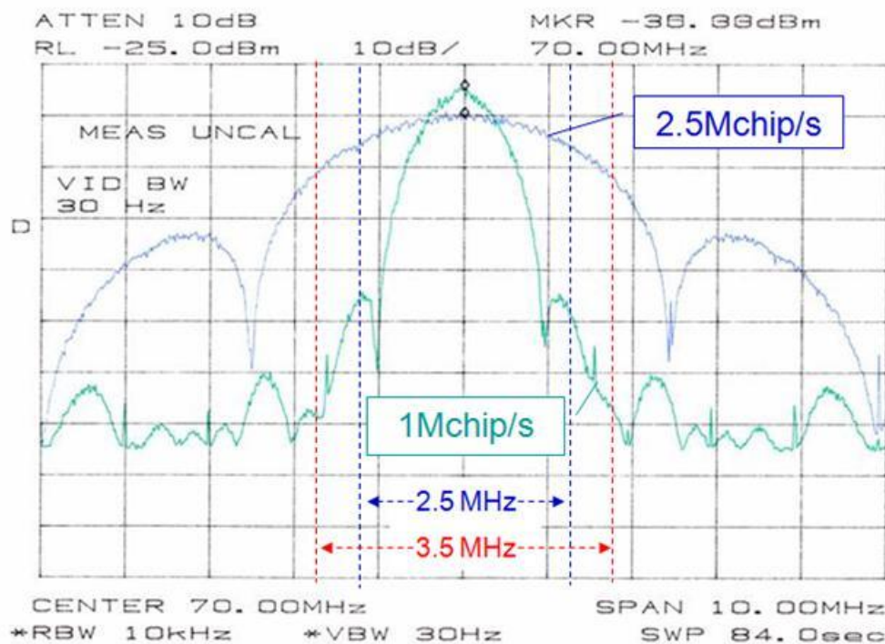
Figure 1. 1 MChip/s and 2.5 MChip/s TX IF spectrum signals.
