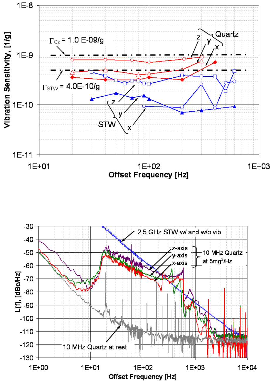
Figure 4. PM noise of the 2.5-GHz STW oscillator is shown in the topmost straight, smooth plot. The 10-MHz quartz oscillator is shown in the bottommost plot. Also shown are the PM noise plots when both oscillators are subject to 20 Hz to 600 Hz random vibration, rms level of 5 mg 2 /Hz. Note the dramatic increase in noise in the quartz oscillator, while no change occurs in the STW oscillator.
