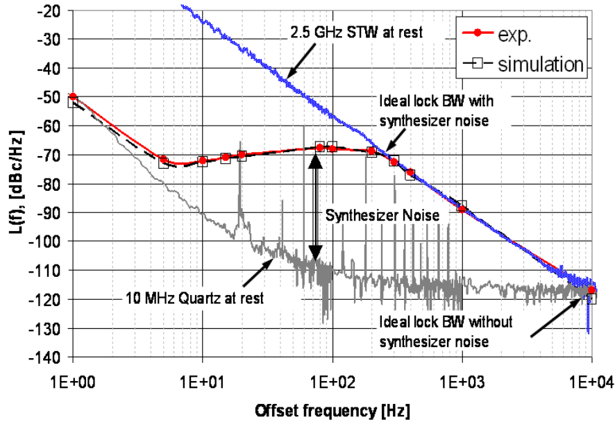
Figure 2. Measured and simulated PM noise of the combined 2.5-GHz and 10-MHz quartz (scaled to 2.5-GHz) oscillators at rest with the scheme shown in Figure 1(a). The frequency synthesizer noise is included. L(f) — single-sideband PM noise.
