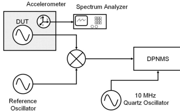
Figure 3. Setup for measuring PM noise and vibration sensitivity of oscillators. DPNMS — Direct digital phase noise measurement system.
