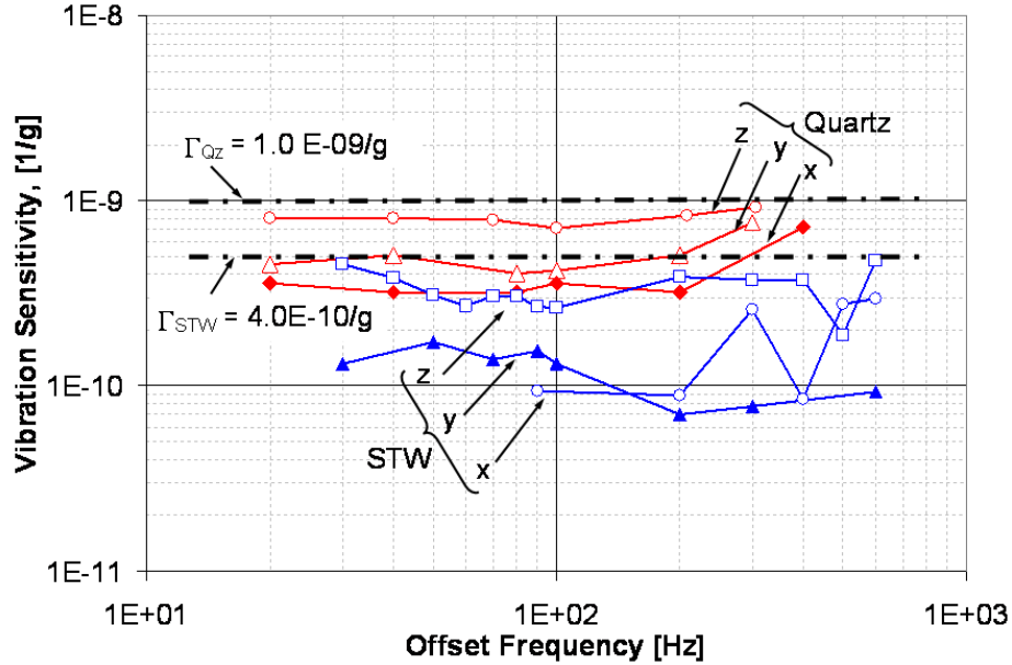
Figure 5. Vibration sensitivity of the 10 MHz quartz and 2.5 GHz STW oscillators along the x, y, and z axes.
