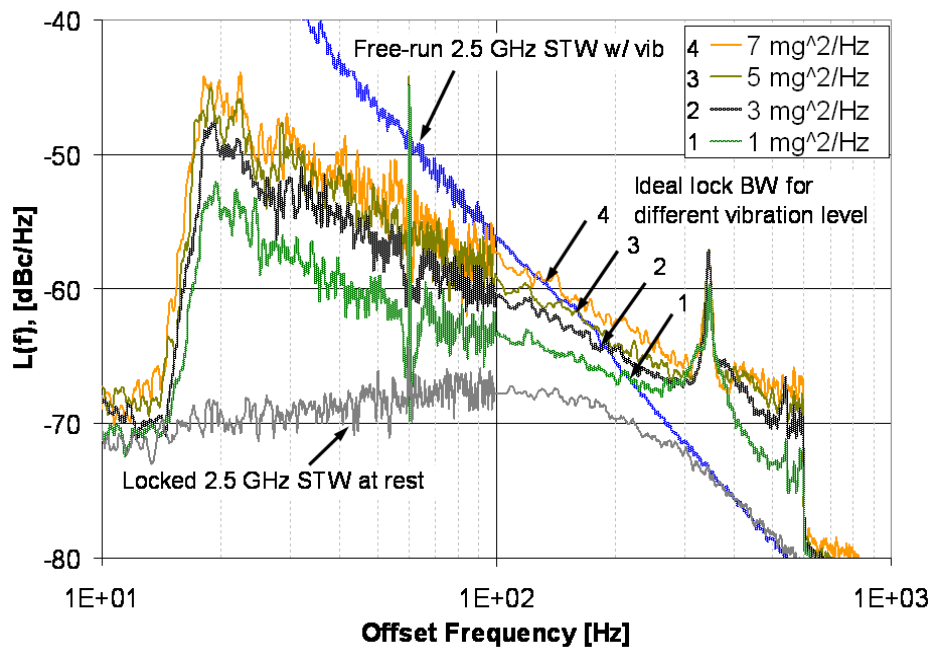
Figure 7. Overall vibration sensitivity of the combined oscillators in the PLL can be reduced by shifting the ideal lock point shown by arrows.
