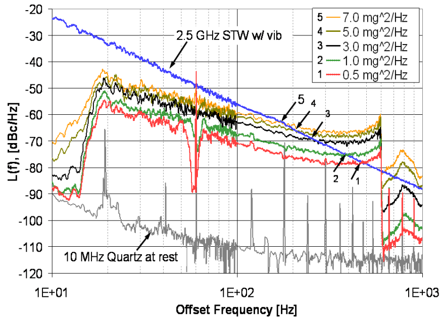
Figure 6. PM noise of free-running oscillators under vibration along the z-axis. Vibration sensitivity of each oscillator causes the optimum PLL BW at f_{cross} shown by arrows to depend on vibration level. A random vibration is applied between 20 \text{ Hz} \leq f_v \leq 10 \text{ kHz} .
