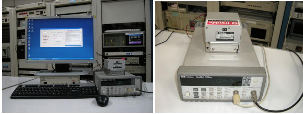
Figure 4. The GPS remote time and frequency calibration system.
