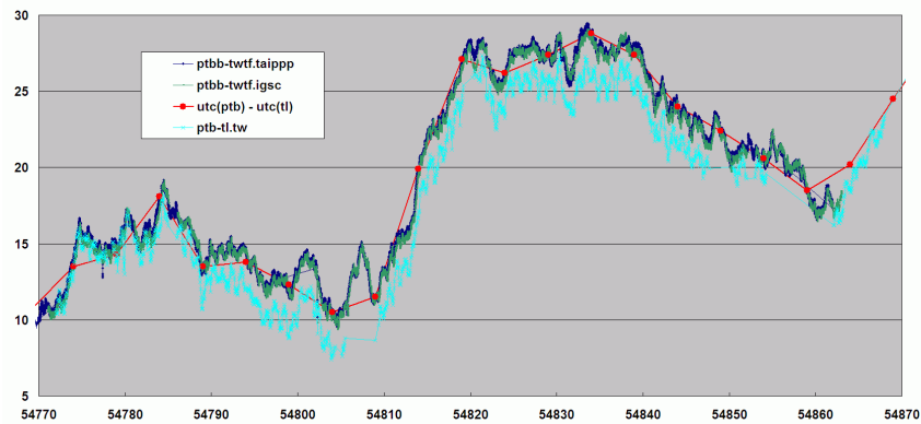
Figure 2. UTC (PTB) – UTC (TL) via different time transfer data.
