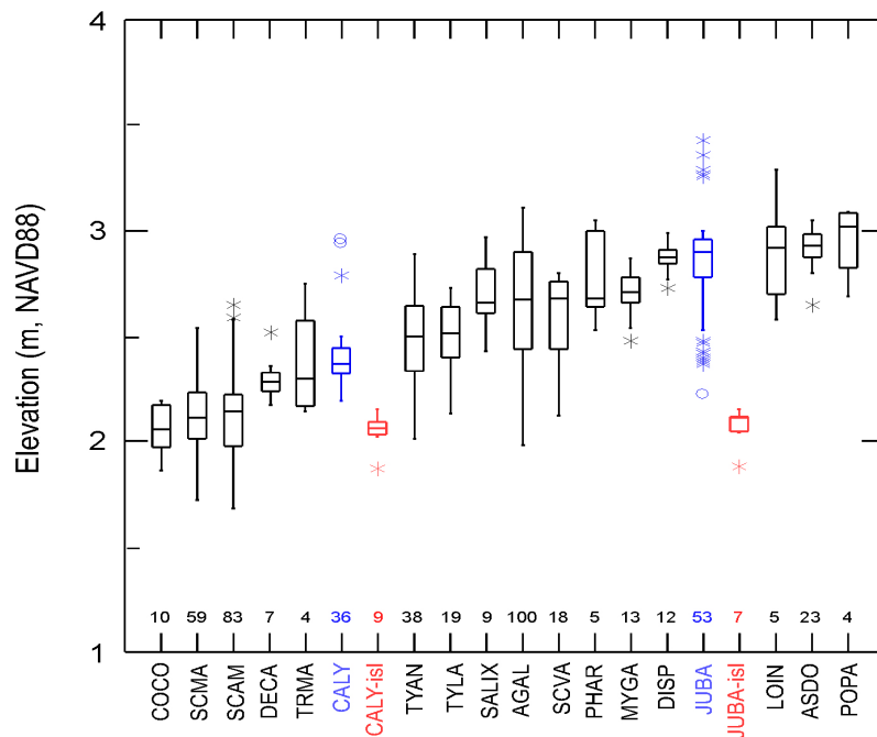
Figure 2. Box plot of preliminary survey of tidal marsh vegetation in the reference marsh (black and blue) vs. newly colonized islands (red). Horizontal bar = median elevation, top box edge = 3rd quartile, bottom box edge = 1st quartile, vertical bars = 1 SD, * = points within 2 SD, 0 = outliers. Sample size appears below each box plot. Carex lyngbyei (CALY) and Juncus balticus (JUBA) appear to be the most common colonizing species and colonize flats at much lower elevations than at which they occur in mature marsh communities.
