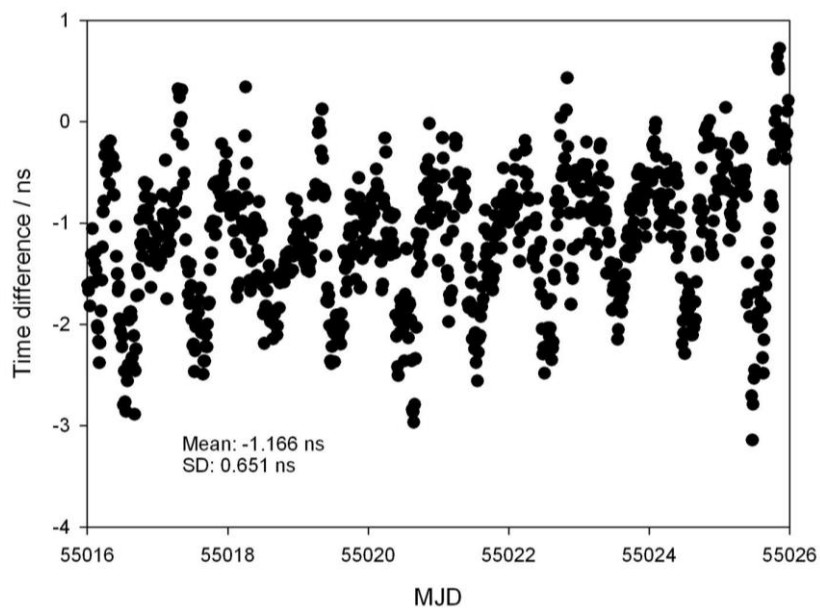
Figure 2. GPS C/A code – TWSTFT + 1.636 ns.
