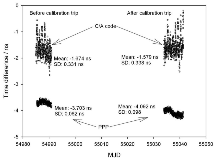
Figure 1. Common clock differences at PTB (TR-PTB07).
