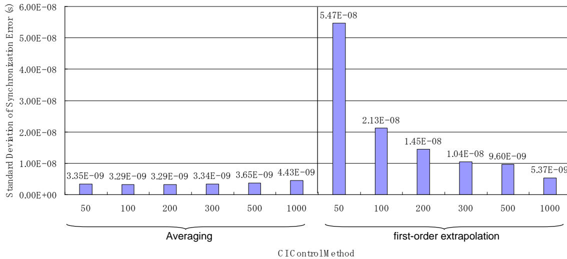
Fig. 7. Standard deviations of maximum synchronization errors (simulation).
