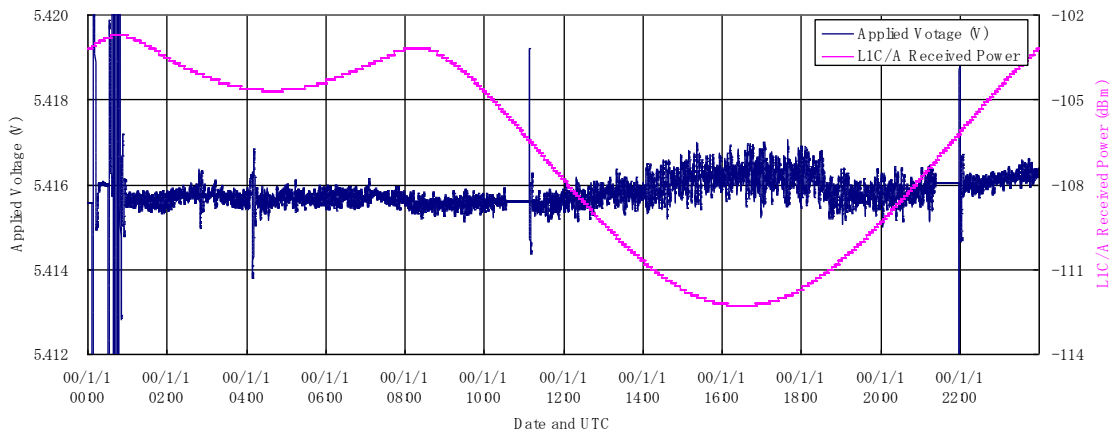
Fig. 13. Result of actual operation experiment (applied voltage and signal power).
