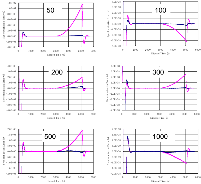
Fig. 6. Simulation results obtained by first-order extrapolation of 50, 100, 200, 300, 500, and 1000 applied voltage data.
