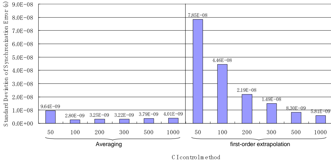
Fig. 11. Standard deviations of maximum synchronization errors (basic experiments).
