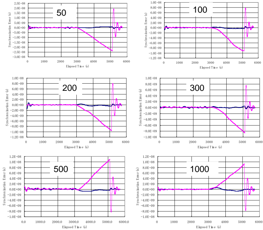
Fig. 9. Basic experimental results obtained by averaging 50, 100, 200, 300, 500, and 1000 applied voltage data.
