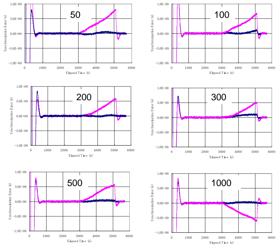
Fig. 5. Simulation results obtained by averaging 50, 100, 200, 300, 500, and 1000 applied voltage data.
