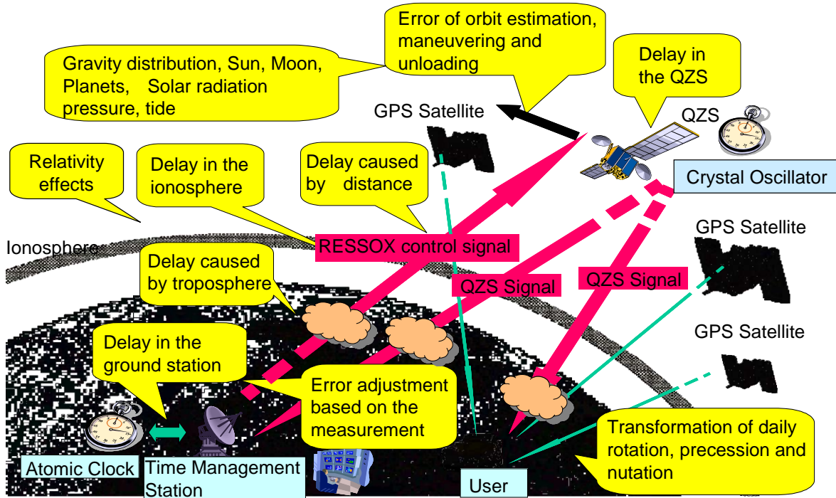
Fig. 1. RESSOX schematic.
