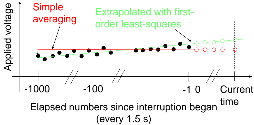
Fig. 2. Schematic of the control method.
