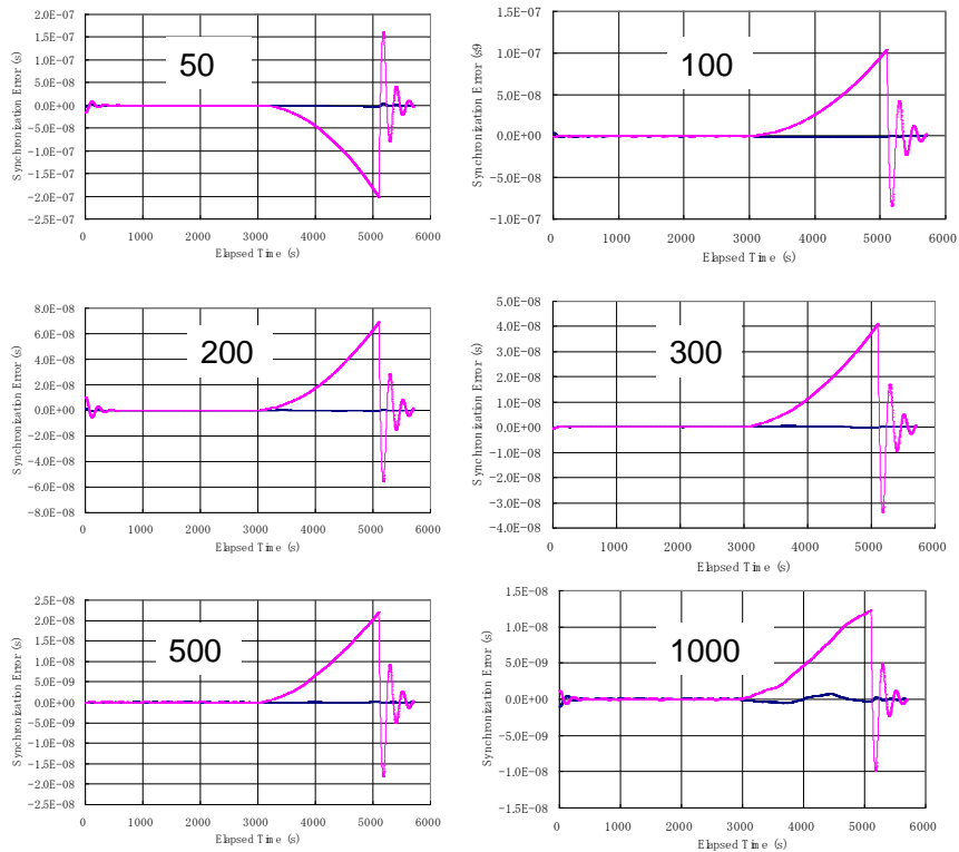
Fig. 10. Basic experimental results obtained by first-order extrapolation of 50, 100, 200, 300, 500, and 1000 applied voltage data.
