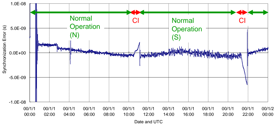
Fig. 12. Result of actual operation experiment (synchronization error).
