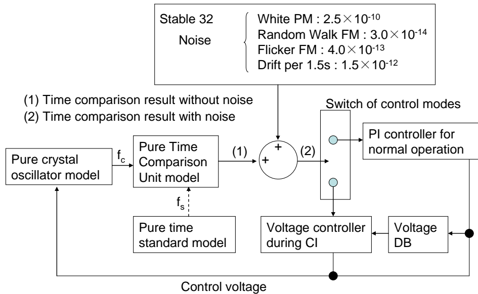
Fig. 3. Block diagram of computer simulation.
