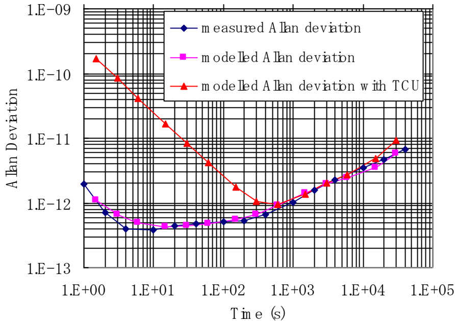
Fig. 4. Allan deviations of actual crystal oscillator, modelled crystal oscillator, and modelled TCU output.
