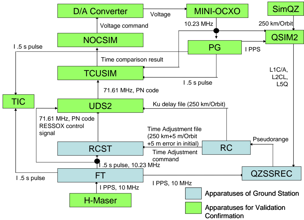
Fig. 8. Block diagram of experimental apparatuses.
