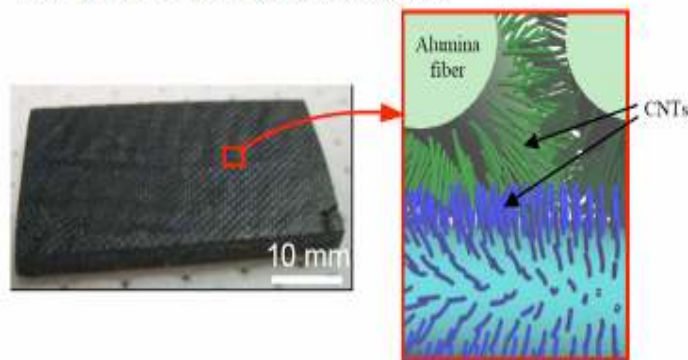
Figure 1. Laminate composed of cloth containing fibers (in tow form) with in situ -grown aligned CNTs in a polymer matrix (left), and illustration of cross-sectional region between tows (right). CNTs grown on the surface of each fiber interact with CNTs of nearby fibers achieving inter-tow and interlaminar reinforcement 3 .
