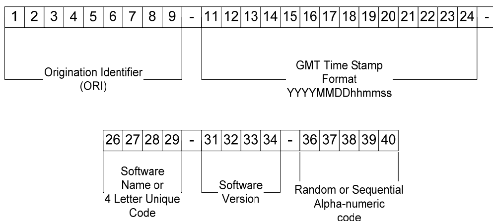
Figure 2: TCN Layout
