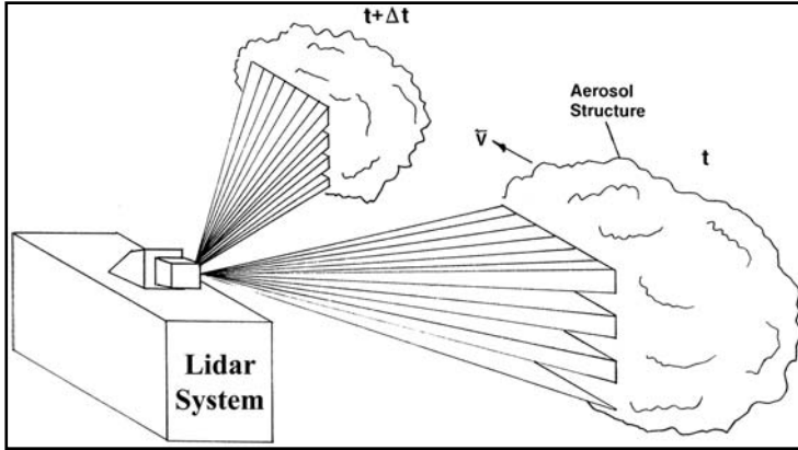
FIGURE 5 The lidar scans back and forth, mapping large aerosol structures (100 m to 1 km) and tracking their movement.
