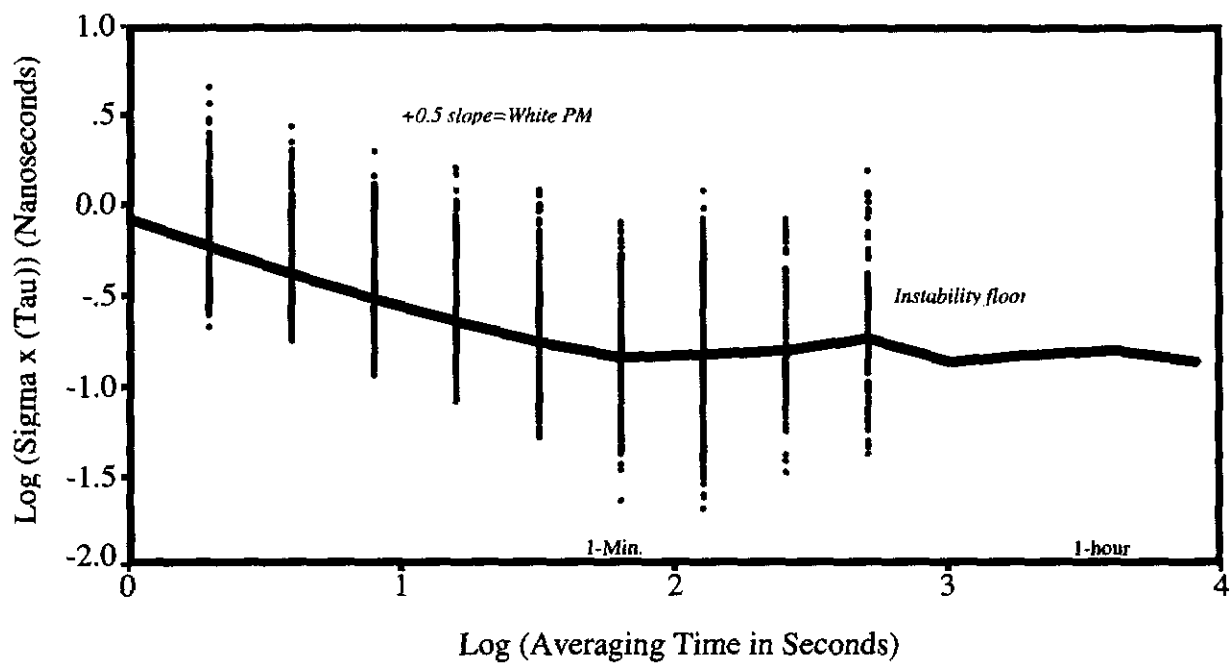
Figure 1. Time-domain instability estimates of 1,492 MITREX modem experiments.
