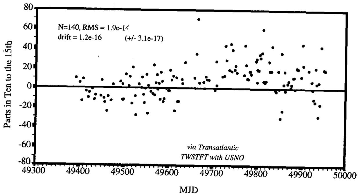
Figure 5. UTC(PTB)-UTC(NPL) via transatlantic TWSTFT with USNO.
