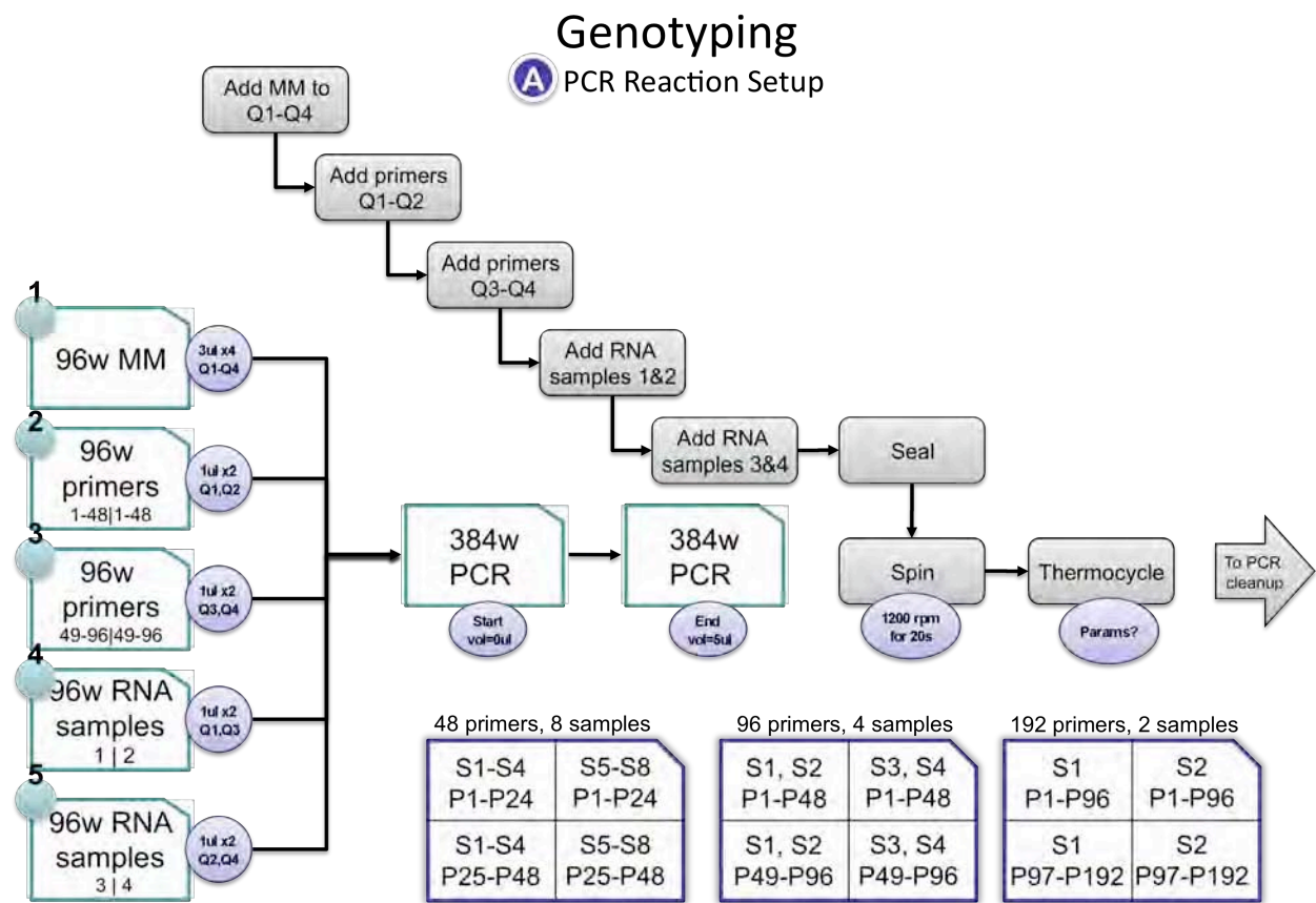
Figure 25. PCR setup step. RT-PCR and PCR are carried out in a one step process using Qiagen's OneStep RT-PCR kit. One microliter of RNA and 1ul total of forward and reverse primers are added to 3ul of master mix in a 384 well plate. The plate is sealed, spun down, and put into a thermal cycler for amplification. Lower three frames depict three possible scenarios of plate layouts with 48, 96 or 192 primers.
