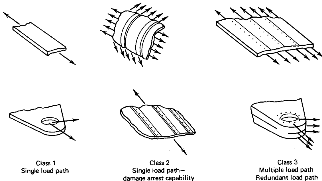
Figure 1: Structural types based on load path [5]
