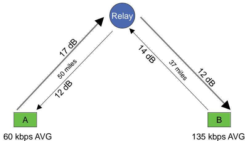
FIGURE 3 Example of 802.11b relay/router testing for two nodes conducting bi-directional multicast. The S/N ratios (expressed in dB) were collected at the receive point at each node in the link.
