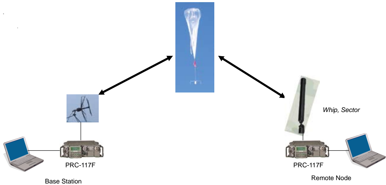
FIGURE 2 Test configuration, UHF high altitude transponder.
