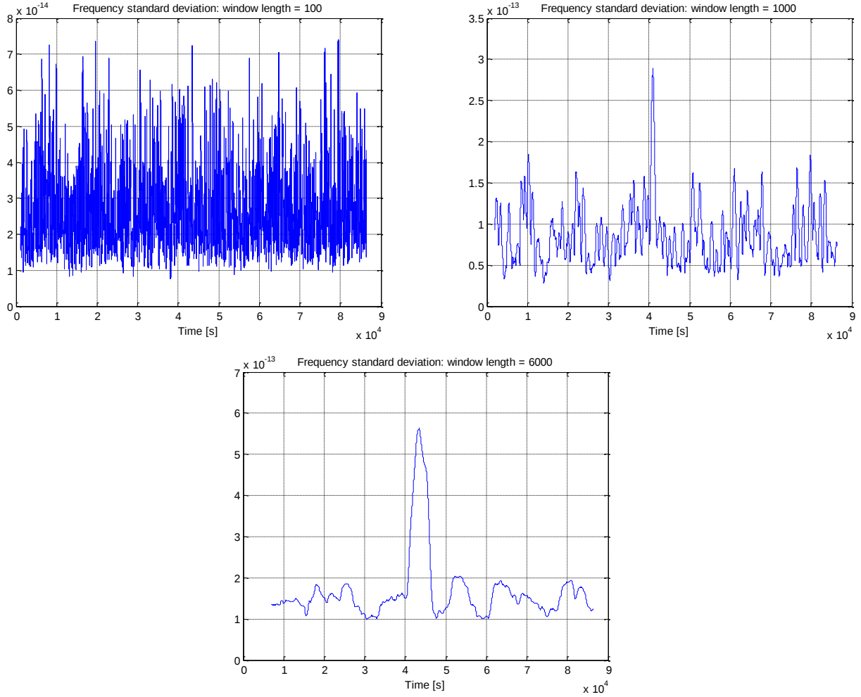
Figure 7. Comparison of test results for \text{len\_fr} <, =, \text{ and } > \tau_{\text{fr}} (1000 s) by StdDev for the frequency jumps of 1 \times 10^{-12} @ 40,000 s by a RAFS.
