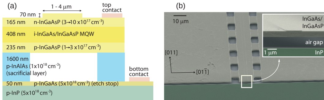
Fig. 1. (a) : The epitaxial layer structure and waveguide rib dimensions (not to scale). (b) : A false-color SEM image of a suspended quantum well waveguide comprised of a shallow rib bounded by etch holes, prior to the deposition of the metal contacts. Inset: the facet of a 2 \mu m wide rib.
