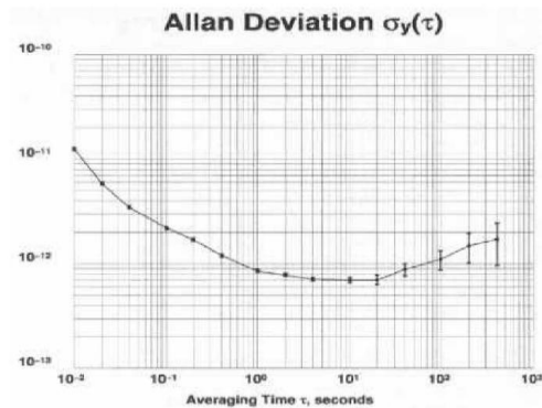
Figure 4. MV89 OCXO, 10 MHz output stability, stand-alone.
