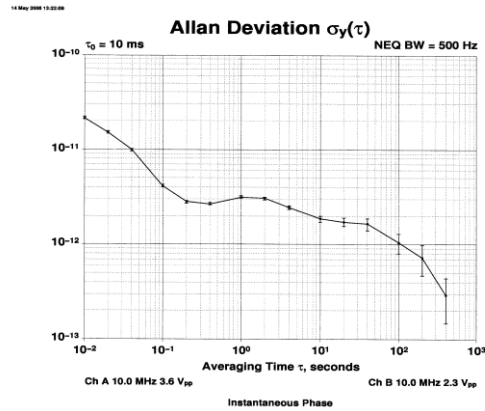
Figure 6. OCXO locked to Rb.
