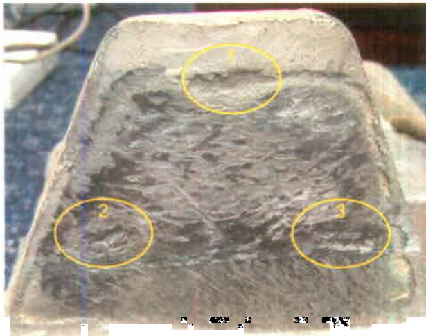
Fig. 15: Used tank shoe with surface cracks
