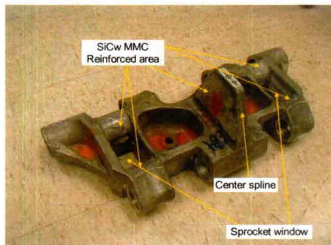
Fig. 1: Tank track shoe to be inspected.
