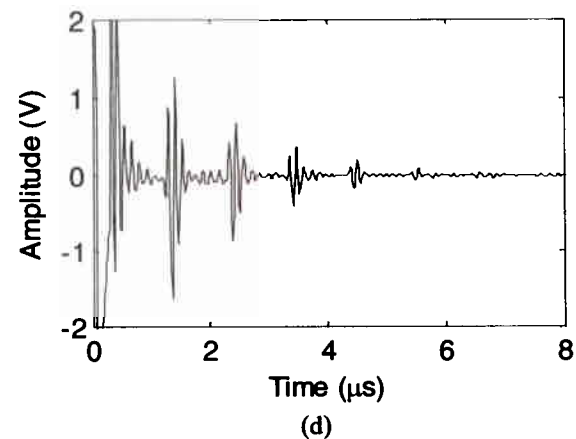
Fig. 2: Illustration of pulse-echo method for disbond detection. (a) Conventional contact transducer on the tank shoe; (b) Illustration of the ultrasound paths; (c) Signal at location with no disbond; (d) Signal at location with disbond.
