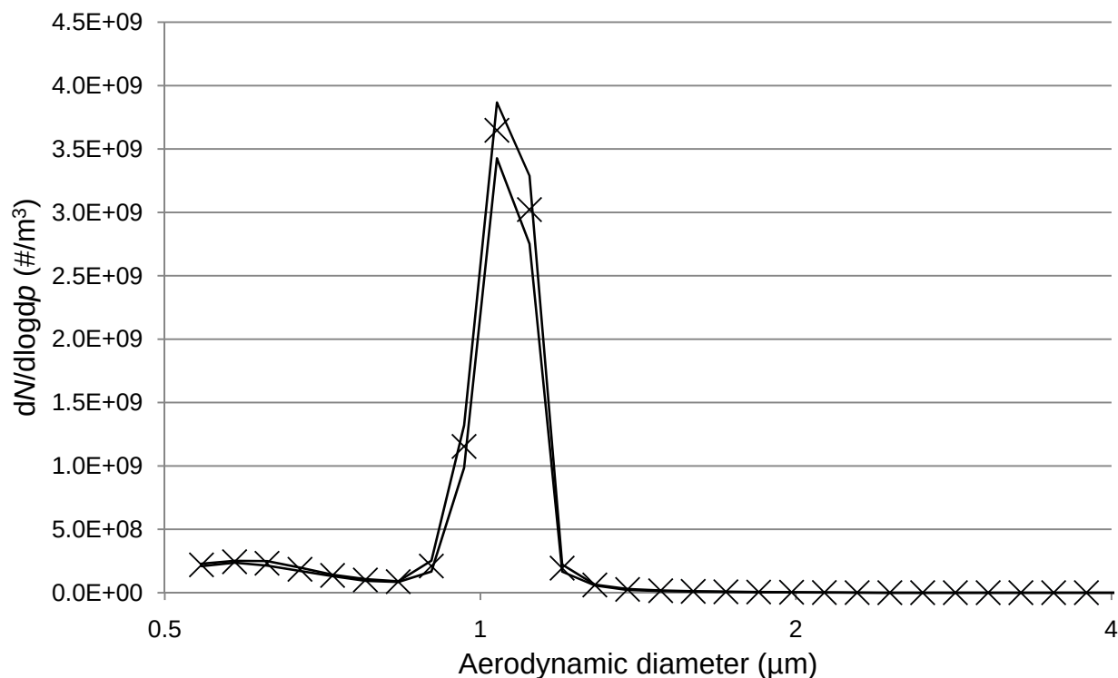
Figure C-2. Representative PSDs from nebulizing 1- \mu\text{m} beads. Data is based on samples taken at quadrants of the mouse tree. Lines are 95% confidence intervals. A broad, slightly unsymmetrical peak consistently occurred at 1.037 \mu\text{m} .
