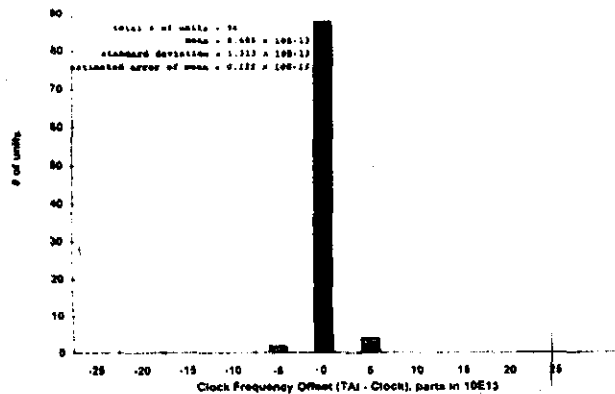
HISTOGRAM OF FREQUENCY OFFSETS (TAI - CLOCK) FOR 1994 (ALL 6071As)
