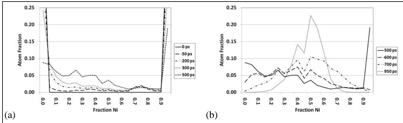
Figure 15. The results here show the fraction of Ni in each alloy at stages (a) 1 and (b) 2 versus fraction of all atoms in each alloy, i.e., a data point at (0.25, 0.1) corresponds to 10% of all atoms in the system belong to \text{Al}_3\text{Ni} .
