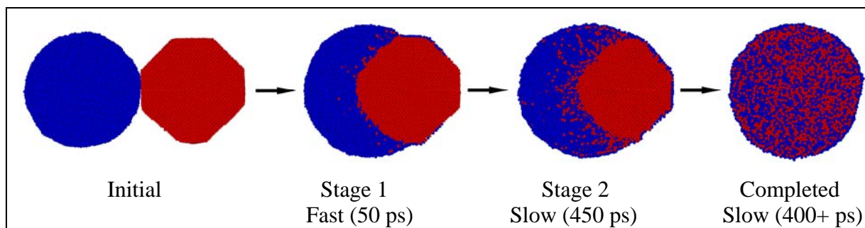
Figure 6. Cross-sectional view from MD simulations of Ni/Al nanoparticle sintering process showing the start of the second stage of coalescence where diffusion is the driving force as opposed to contact area maximization. Al atoms are blue and Ni atoms are red.
