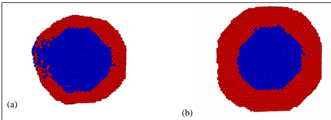
Figure 14. Cross sections of the Ni-coated Al nanoparticle simulation model just after melting of the Al core for the (a) 1-nm-thick and (b) 2-nm-thick Ni shells.
