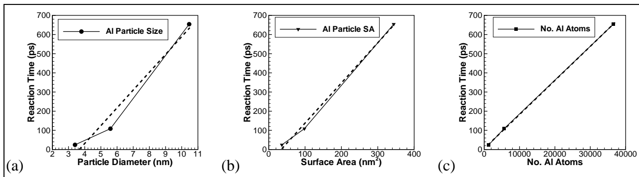
Figure 9. Reaction time versus (a) Al nanoparticle diameter, (b) Al nanoparticle surface area, and (c) number of Al atoms. Note the nearly linear relationship (dashed line) of reaction time between number of atoms (volume) and surface area.
