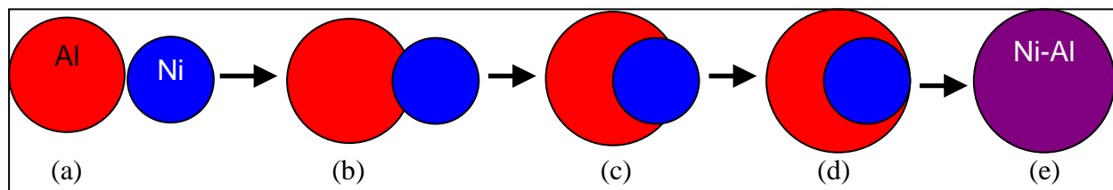
Figure 1. Illustration of sintering process showing liquid Al nanoparticle first coating the solid Ni nanoparticle and then complete alloying after the Ni nanoparticle has melted.
