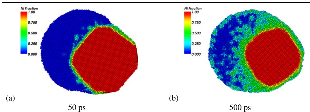
Figure 16. Plot showing spatial distribution of Ni fractions during stages (a) 1 and (b) 2 of the sintering process.
