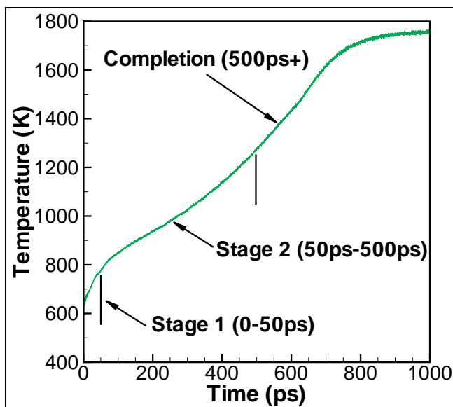
Figure 7. Time vs. temperature plot for sintering of separate 10-nm-diameter Al and Ni nanoparticles. The various stages of the coalescence processes are denoted on the curve, including the final completion stage that occurs after the Ni nanoparticle has melted.
