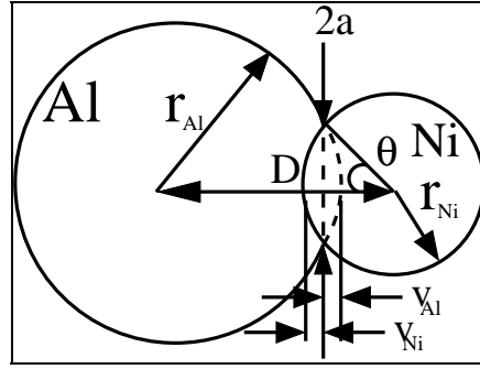
Figure 2. Illustration of parameters used in analytical model of reactive coalescence of Ni and Al nanoparticles.
