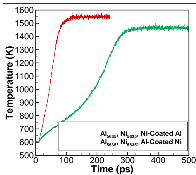
Figure 13. Comparison of combustion temperature for Ni-coated Al nanoparticle versus Al-coated Ni nanoparticle.
