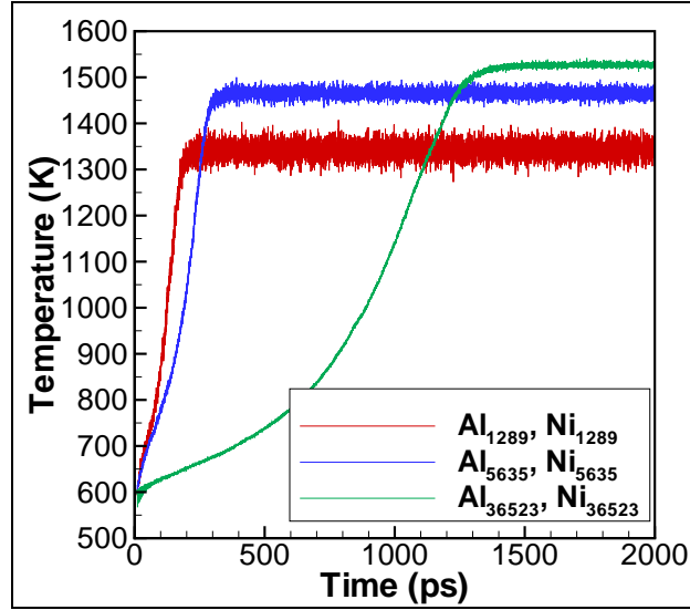
Figure 10. Temperature vs. time in the sintering of Al-coated Ni nanoparticles with an Ni:Al ratio of 1:1.
