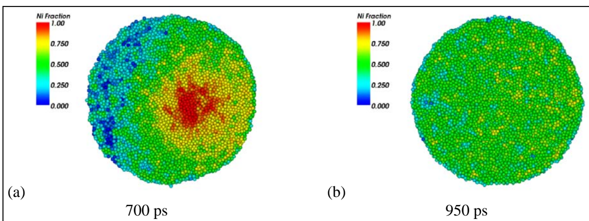
Figure 17. Plot showing spatial distribution of Ni fractions at the (a) beginning and (b) end of stage 3 of the sintering process.
