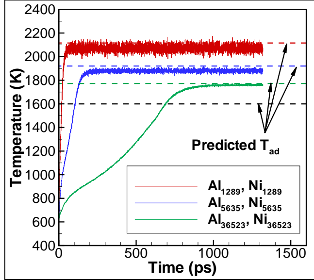
Figure 8. Temperature vs. time in the sintering of nanoparticles with an Ni:Al ratio of 1:1.
