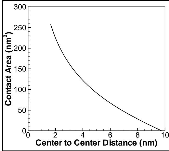
Figure 4. Contact or interface area as a function of center-to-center distance. The contact area is increasing as the nanoparticles move closer together (right to left on x-axis).
