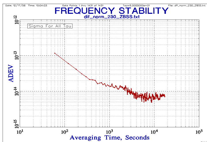
Fig. 3. ADEV by GPSCP in the zero-baseline experiment with the same reference.
