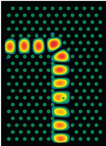
FIGURE 2 EBG waveguide showing a narrow-band transient bending around a sharp corner.
