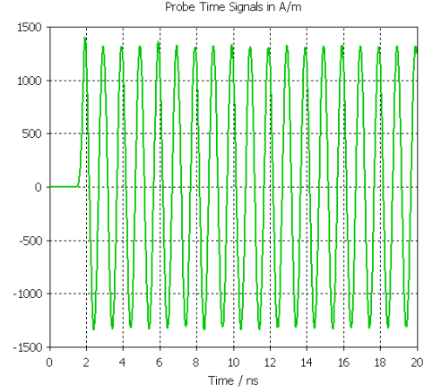
(b) H-field at z = 0.0m inside the FSS aperture.
