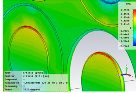
(b) z - axis electric field distribution on radius edged ring element.
