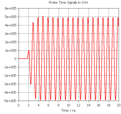
(d) E-field at z = -250mm on the transmitted side of FSS.
