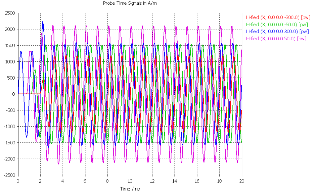
Figure 4.18: Magnetic field strength for silver/aron FSS. As in the electric field before, the transmitted and the incident/reflected waves are both affected by the lossy material properties.
