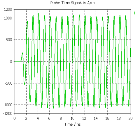
(c) H-field at z = -50mm on the transmitted of FSS.
