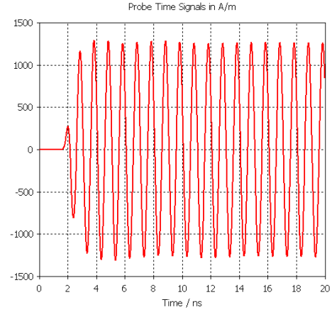
(d) H-field at z = -250mm on the transmitted of FSS.
