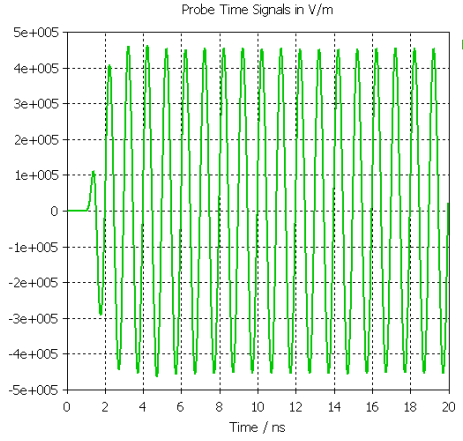
(c) E-field at z = -50mm on the transmitted side of FSS.
