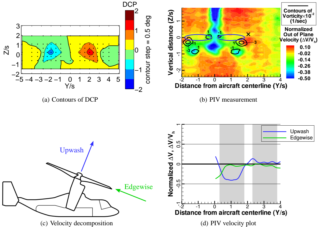
Figure 9. Formation flight at 80 knots full-scale, 1000 \text{ ft}/\text{min} descent, C_T = 0.010 , x/D = 2.818
