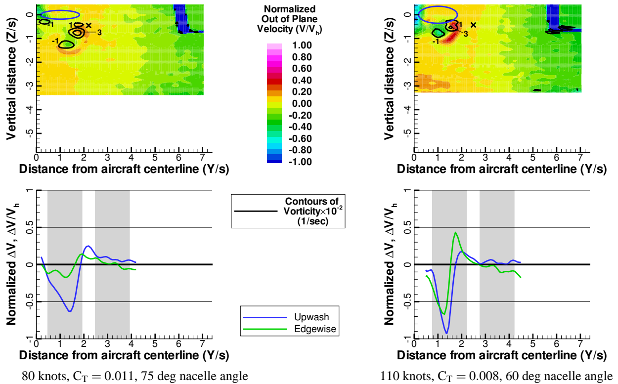
Figure 11. PIV measurements for various flight speeds. Level flight. x/D = 2.818
