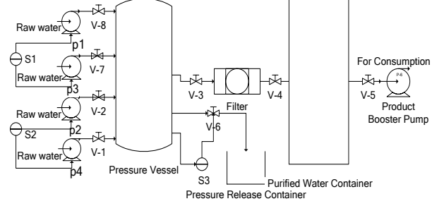
Figure 6 A Simplified Water Treatment System
