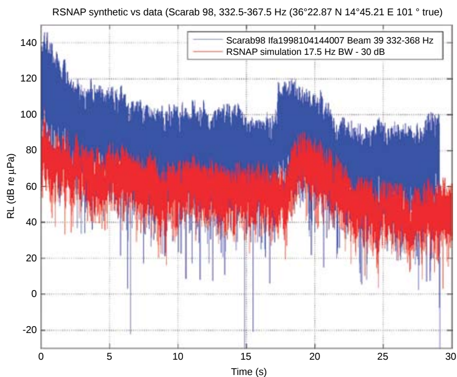
FIGURE 3 Narrowband reverberation time series in the 332–368 Hz band measured from the Ragusa Ridge on the Malta Plateau during SCARAB 98 (blue), and simulated by R-SNAP for the same frequency band (red, offset by 30 dB) using environmental parameters measured in situ. The simulation captures many of the characteristics of the measured data.
