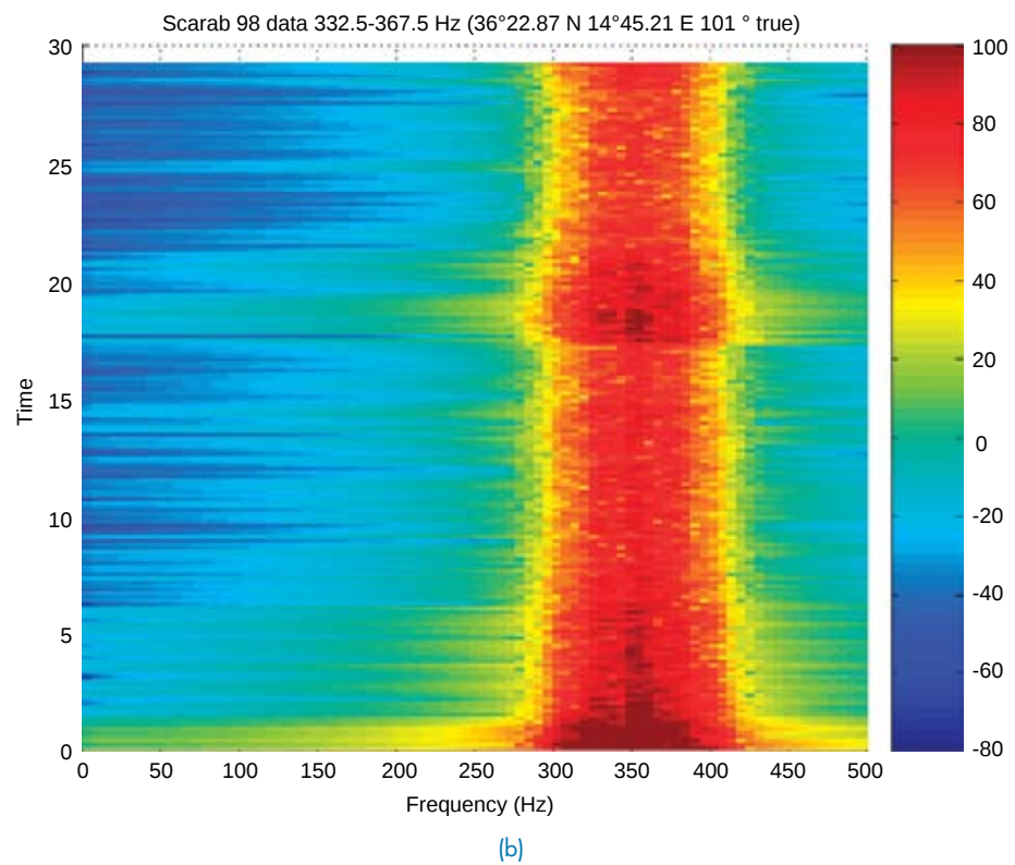
FIGURE 4 Spectrograms of (a) 350 Hz R-SNAP simulation shown in Fig. 3, and (b) SCARAB 98 data. Many of the characteristics of the data are captured by the simulation, including coherent time-frequency striations of positive slope and the clutter return from the Ragusa Ridge starting at 18 s.
