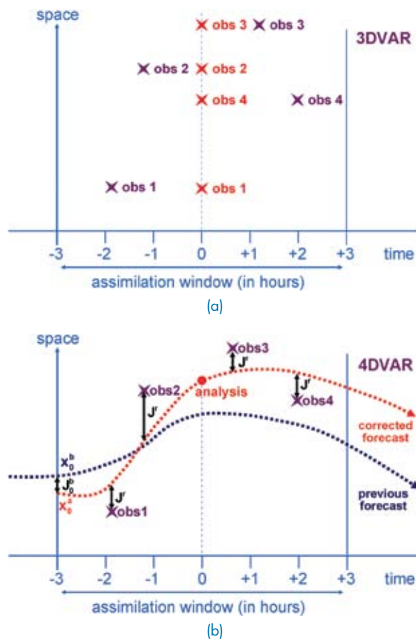
FIGURE 4 A schematic of 3DVAR (a) and 4DVAR (b). The abscissa represents time of the data assimilation. The ordinate indicates the observation locations in three-dimensional space. Four observations (obs 1 – obs 4) are scattered at different temporal and spatial locales over the 6-hour data assimilation time window. (a) In 3DVAR, all observations are assimilated at “0” hour and the results are constrained by simple geophysical relationships. (b) In 4DVAR, all observations are assimilated at the “observed” hours and the dynamical model is used to constrain the results.
