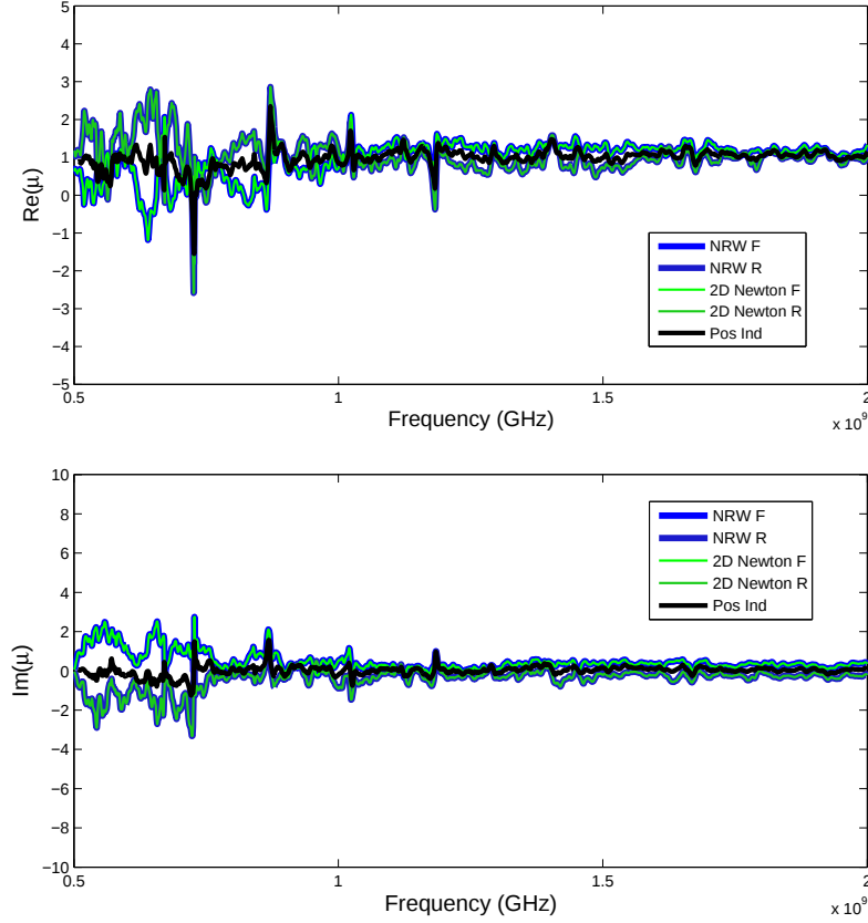
Figure 4.4: Real and Imaginary Components of Fiberglass Permeability
