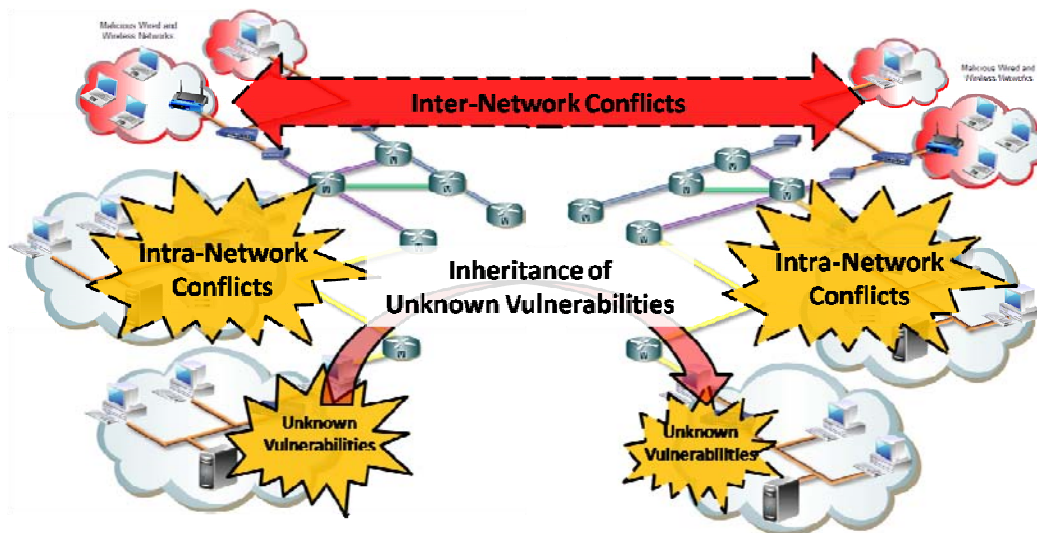
Figure 5. System-level Vulnerabilities
