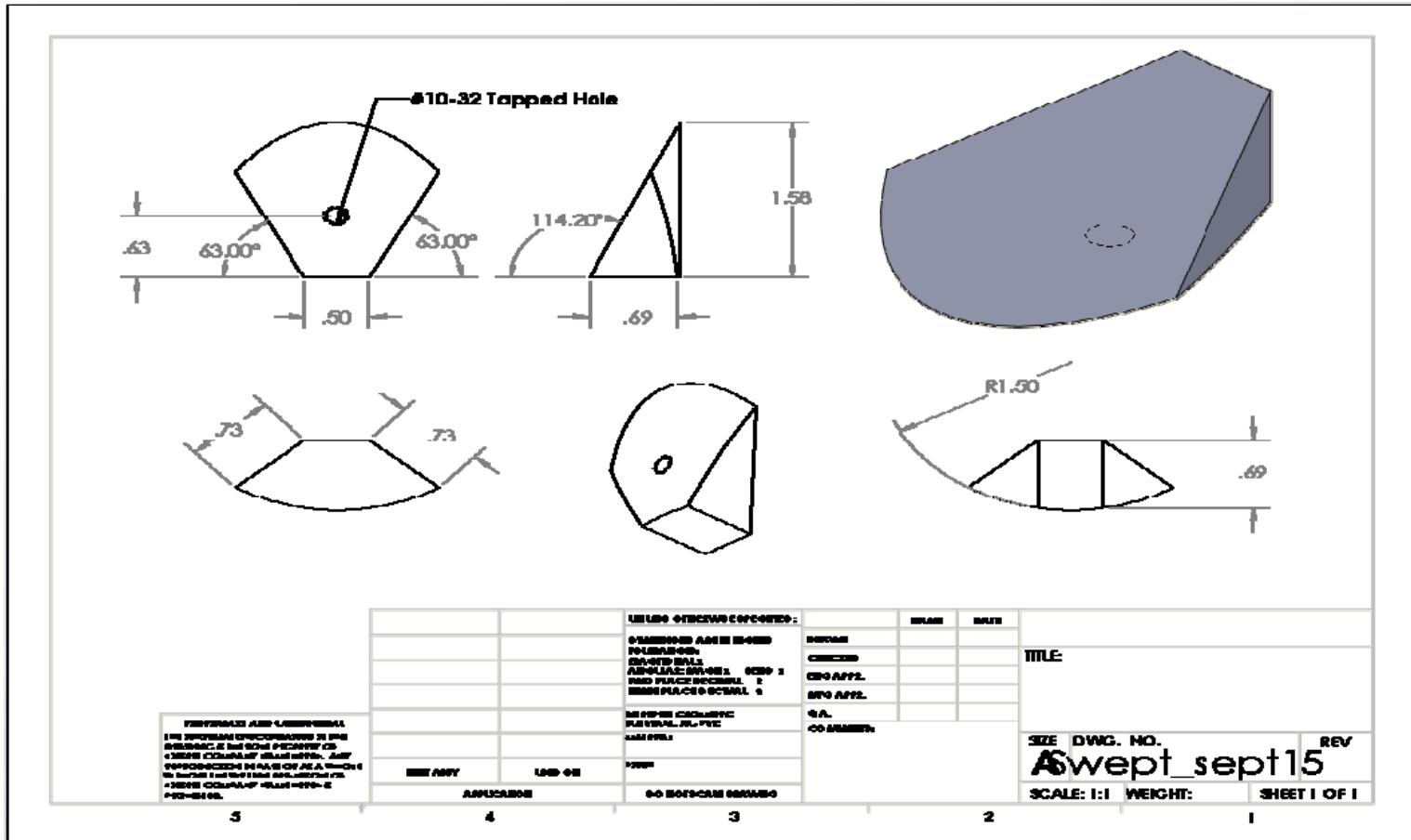
Figure 47. Tall swept
