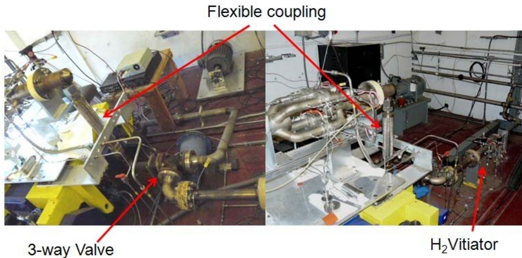
Figure 36. Flexible coupling
