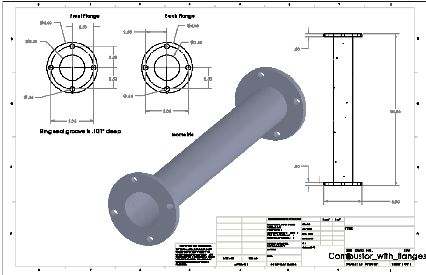
Figure 45. Combustor drawing
