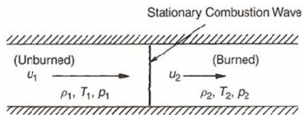
Figure 3. Schematic diagram of stationary 1-D combustion wave [From 1]
