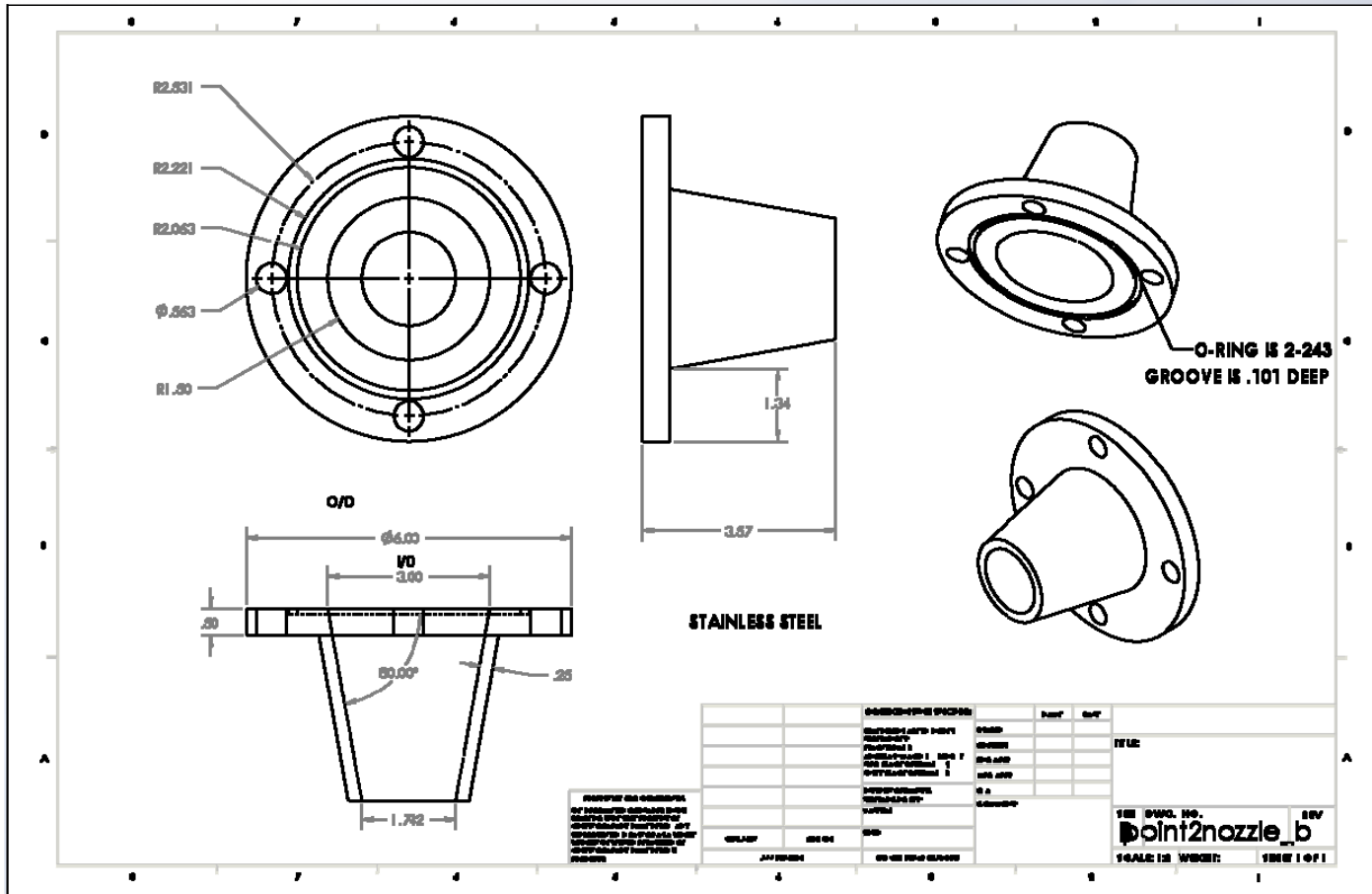
Figure 46. 0.2 Mach nozzle
