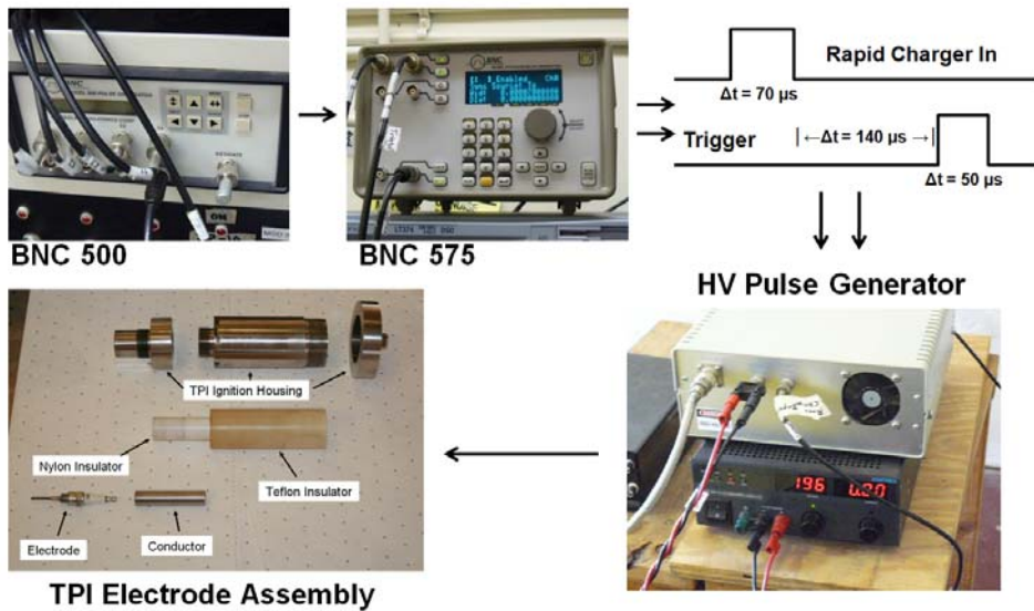
Figure 20. Signal path for transient plasma ignition
