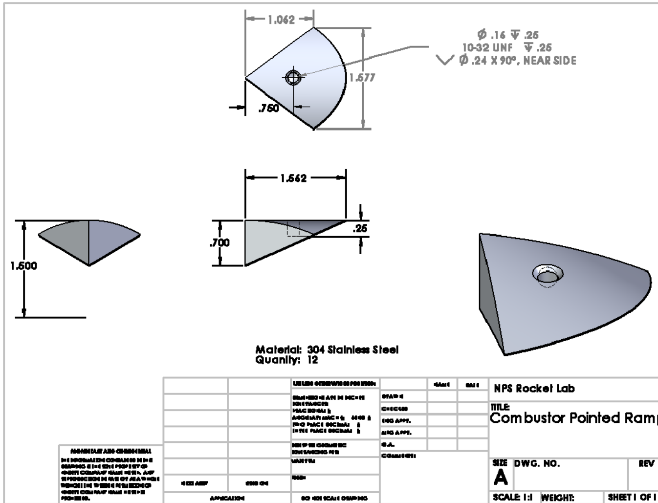
Figure 51. Pointed ramp
