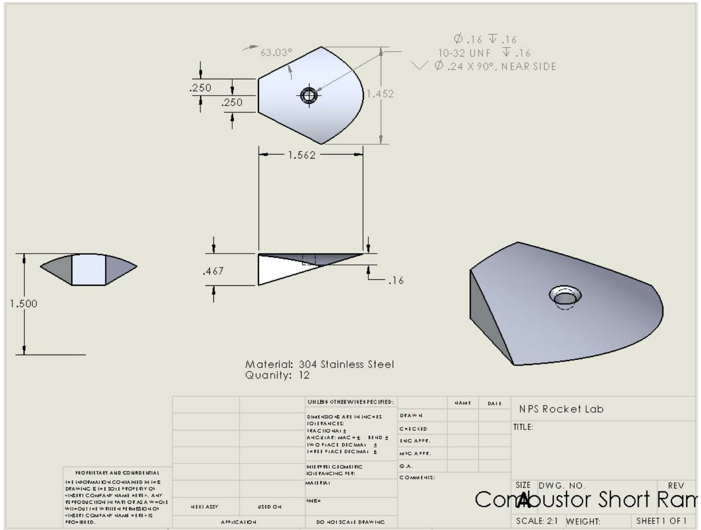
Figure 48. Short swept
