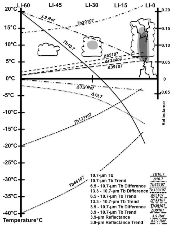
Figure 39. Conceptual model of LI IF behavior in the hour preceding first lightning, adapted from MB06. Typically, no cloud exists at LI-60. Cumuli begin to appear by LI-45, and precipitation—the gray shading—often forms within the cloud once the CTT reaches about 273 K. Lightning initiates at LI-0. 15-minute trend IFs are indicated by \Delta .
