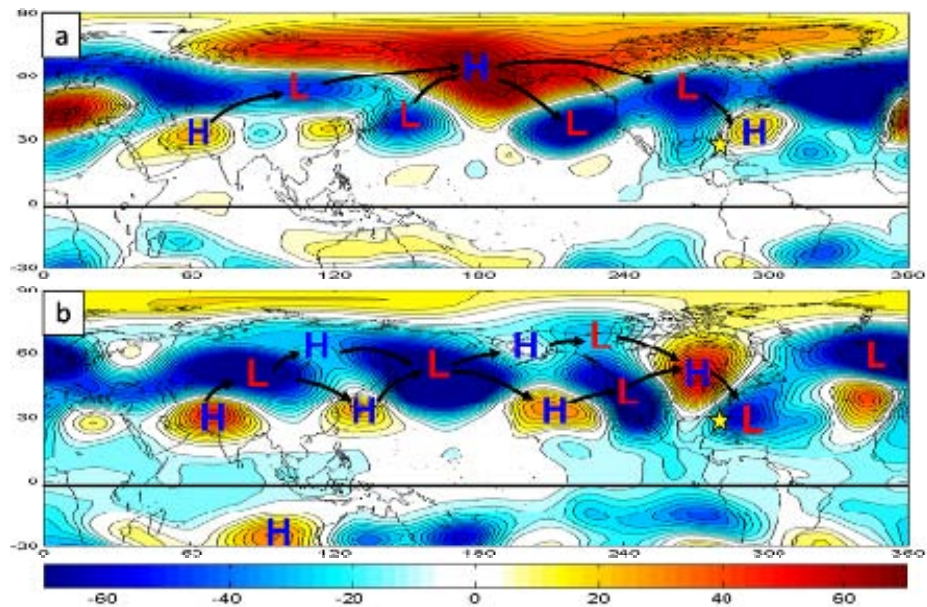
Figure 32. Composite 200 mb GPH anomalies (m) for the ramp-down II season during the three years in which there were: (a) above normal lightning violations; and (b) below normal lightning violations. Anomalous Rossby wave trains that extend over the SE U.S. are marked with H and L, and black arrows. The H and L identify the centers of the positive (negative) height anomalies that help define the wave trains. The black arrows link the centers that are part of individual wave trains and indicate the direction of anomalous energy propagation in the wave trains. The yellow stars indicate the location of the Florida Peninsula.
