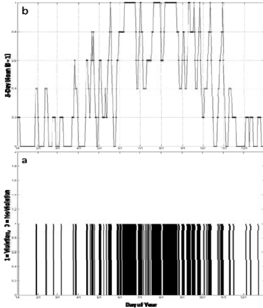
Figure 7. (a) Violation days and (b) 5-day mean of violation days for a representative year. A violation day in panel (a) corresponds to a value of 1.0, meaning there was at least one lightning strike during the day. Values in panel (b) were calculated from data in panel (a). Results from both panels were used to define lightning violation seasons.
