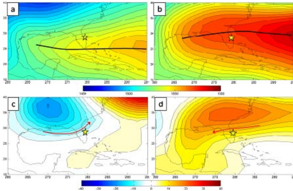
Figure 45. Composites of 850 mb GPH (m). The panels on the left (a, c) represent conditions during the first ten days following an early start of the main lightning violation season. The panels on the right (b, d) represent conditions during the ten days immediately prior to late start dates of the main lightning violation season (late starts). Panel (a) is the composite 850 mb GPH for the first ten days after the early start dates of the main lightning violation season; panel (b) is the composite 850 mb GPH for the ten days prior to the late start dates of the main lightning violation season; panel (c) is the composite 850 mb GPH anomaly for the first ten days after the early start dates of the main lightning violation season; and panel (d) is the composite 850 mb GPH anomaly for the ten days prior to the late starts of the main lightning violation season. The bold black lines show the axis of the ridge at 850 mb with red arrows representing anomalous 850 mb flow. Yellow stars indicate the approximate location of KSC/CCAFS.
