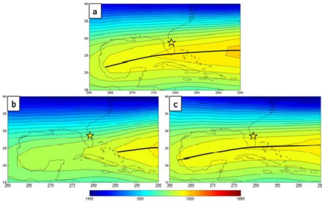
Figure 33. 850 mb GPH (m) for the lightning winter season: (a) LTM; (b) composite mean for the three years with above normal number of lightning violation (see Table 6); and (c) composite mean for the three below normal number of lightning violation years. The bold black lines indicate the position of the 850 mb ridge axis. The yellow star indicates the approximate location of KSC/CCAFS.
