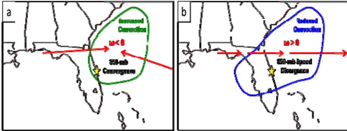
Figure 19. Schematic diagram of regional conditions associated with above normal (panel a) and below normal (panel b) lightning violations during the main lightning season at KSC/CCAFS.
