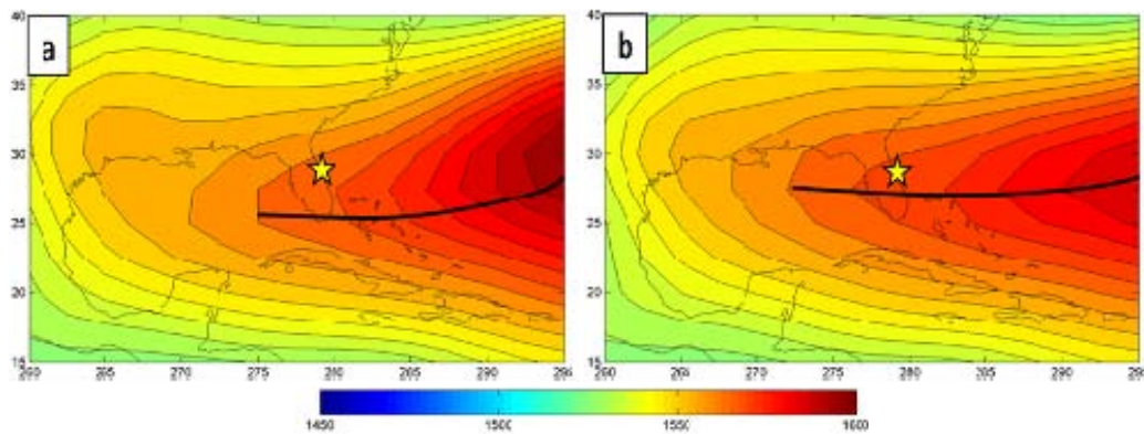
Figure 14. Composite mean 850 mb GPH (m) during the main lightning season for three years (see Table 6) in which there were: (a) above normal lightning violations and (b) below normal lightning violations. The bold black lines show the axis of the ridge at 850 mb. The yellow star indicates the approximate location of KSC/CCAFS.
