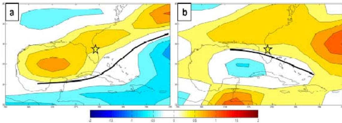
Figure 17. Composite 850 mb zonal wind anomalies (m/s) during the main lightning season for periods in which there were: (a) above normal lightning violations and (b) below normal lightning violations. The bold black lines indicate show the anomalous ridge axis at 850 mb. The yellow star indicates the approximate location of KSC/CCAFS.
