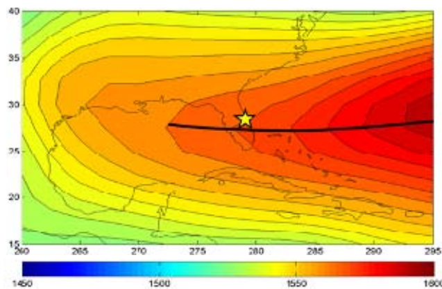
Figure 13. 850 mb LTM GPH (m) for the main lightning season during 1989-2008. The bold black line shows the axis of the ridge at 850 mb. The yellow star indicates the approximate location of KSC/CCAFS.
