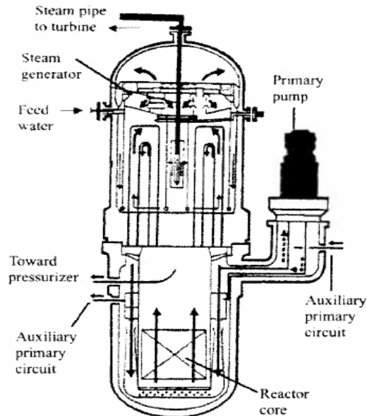
Figure 6. Integrated Reactor and Steam Generator in France's Rubis Nuclear-Powered Submarine. 89
