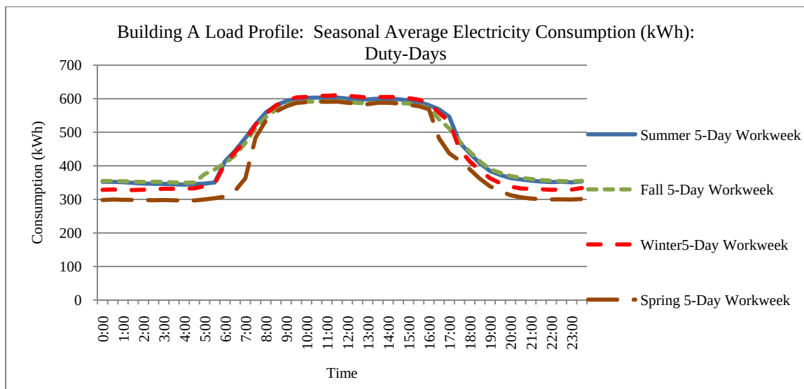
Figure 10. Building A Load Profile: Seasonal Average Electricity Consumption: Duty-Days
