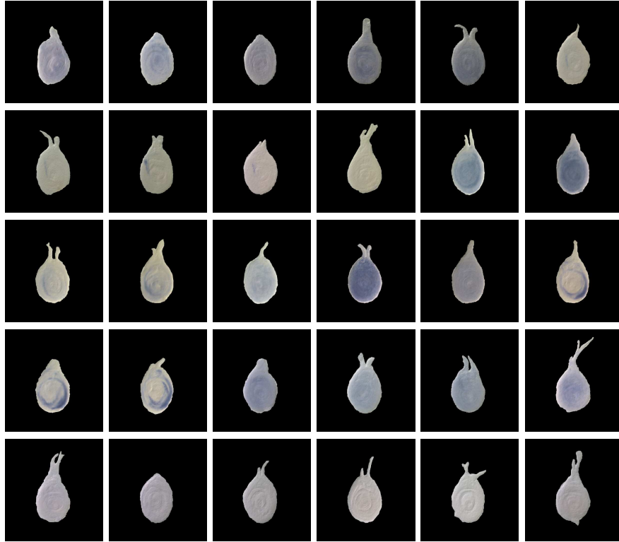
Figure 3.13: Alignment results for leg discs: Segmented leg discs I_a^i after applying the transformations learned by JPA with 7 parameters (Equation (3.9)).
