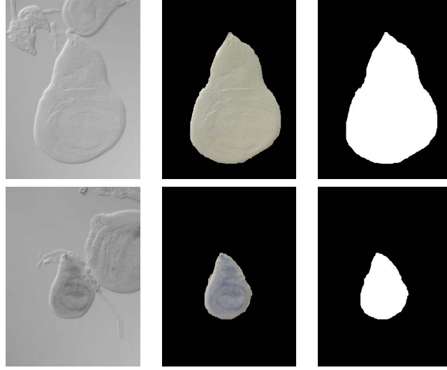
Figure 3.3: Example segmentation results for wing discs (first row) and haltere discs (second row) using the combined segmentation procedure. Left Column: Original image I^i(x) . Middle Column: Segmented tissue structure of interest I_f^i(x) . Right Column: Extracted binary shape I_s^i(x) .
