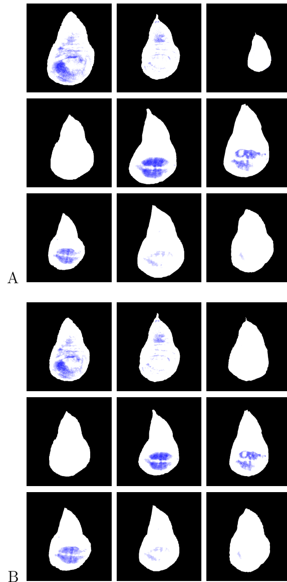
Figure 3.20: Stain patterns in Drosophila imaginal disc images: unaligned vs. aligned. A : Unaligned stain-scored wing disc images. B : Aligned stain-scored wing disc images after JPA. Black pixels have been segmented as background, white indicates no stain and shades of blue indicate stained pixels. Blue intensity values were calculated from the semi-quantitative stain scoring algorithm with the lightest blue representing value 1 and the darkest blue representing value 5. It can be noted that pixel-wise stain count is much more meaningful in these images. (This image is better viewed in color).
