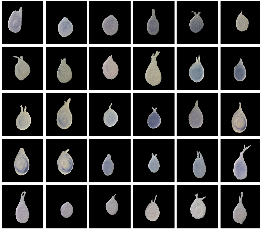
Figure 3.11: Segmented leg discs I_f^i before JPA.
