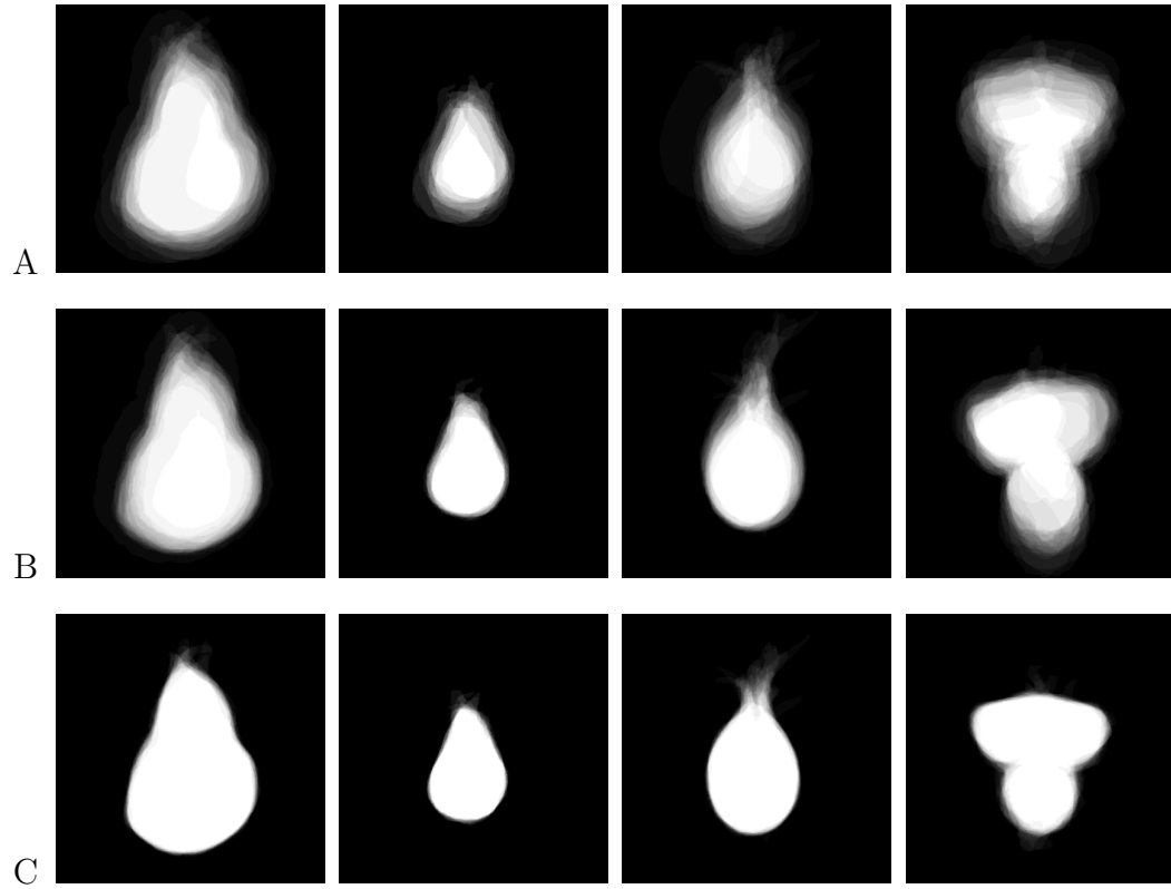
Figure 3.4: Mean shape images from the learning stage. Mean images from optimization process during JPA for wing discs ( first column ), haltere discs ( second column ), leg discs ( third column ), eye discs ( fourth column ): A : Mean image of \Phi_s before JPA . B : Mean image of \Phi_s after JPA to convergence with only 3 parameters ( t_x, t_y and \theta ). C : Mean image of \Phi_s after JPA to convergence with 7 parameters (Equation (3.9)).
