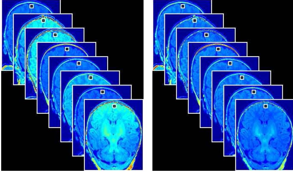
Figure 4.2: Pixel stacks in MR images. On the left are a set of mid-coronal brain images from eight different infants, showing clear signs of bias fields. A pixel-stack, a collection of pixels at the same point in each image, is represented by the small square near the top of each image. Although there are probably no more than two or three tissue types represented by the pixel-stack, the brightness distribution through the pixel-stack has high empirical entropy due to the presence of different bias fields in each image. On the right are a set of images that have been corrected using our bias field removal algorithm. While the images are still far from identical, the pixel-stack entropies have been reduced by mapping similar tissues to similar values in an unsupervised fashion, i.e. without knowing or estimating the tissue types.
